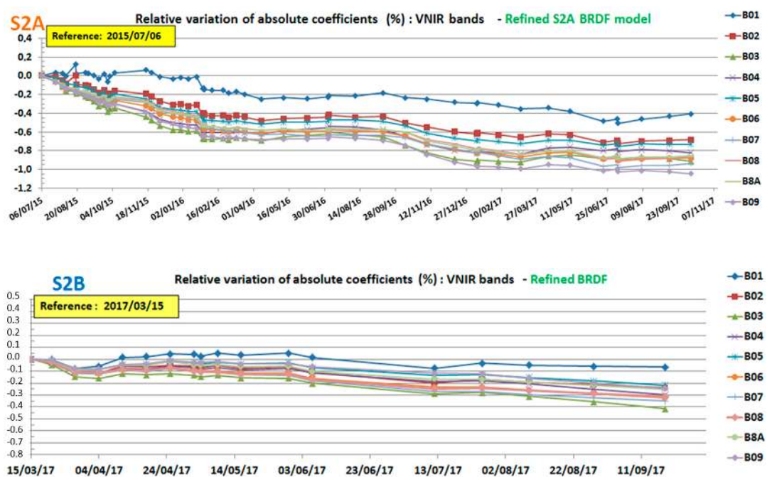
Figure 4. Refined time series of absolute gain coefficients for S2A and S2B based on the improved solar-diffuser bidirectional reflectance distribution function (BRDF) model.
