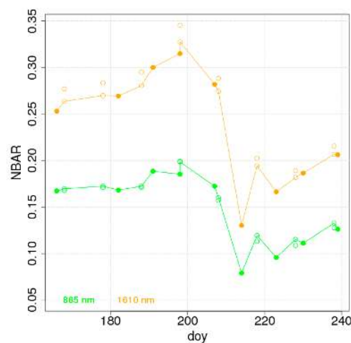
Figure 13. Illustrative time series of Landsat 8 OLI (filled circles) and Sentinel-2A MSI (open circles) atmospherically corrected nadir BRDF-adjusted reflectance (NBAR) for a single 30 m woody savanna pixel location in the 2016 dry season over Zambia (74 days). The open circles without and with an intersecting line show the MSI surface NBAR without and with respectively application of a spectral linear transformation used to adjust the MSI to OLI [52]. The location burned after day 208 and on or before day 214.
