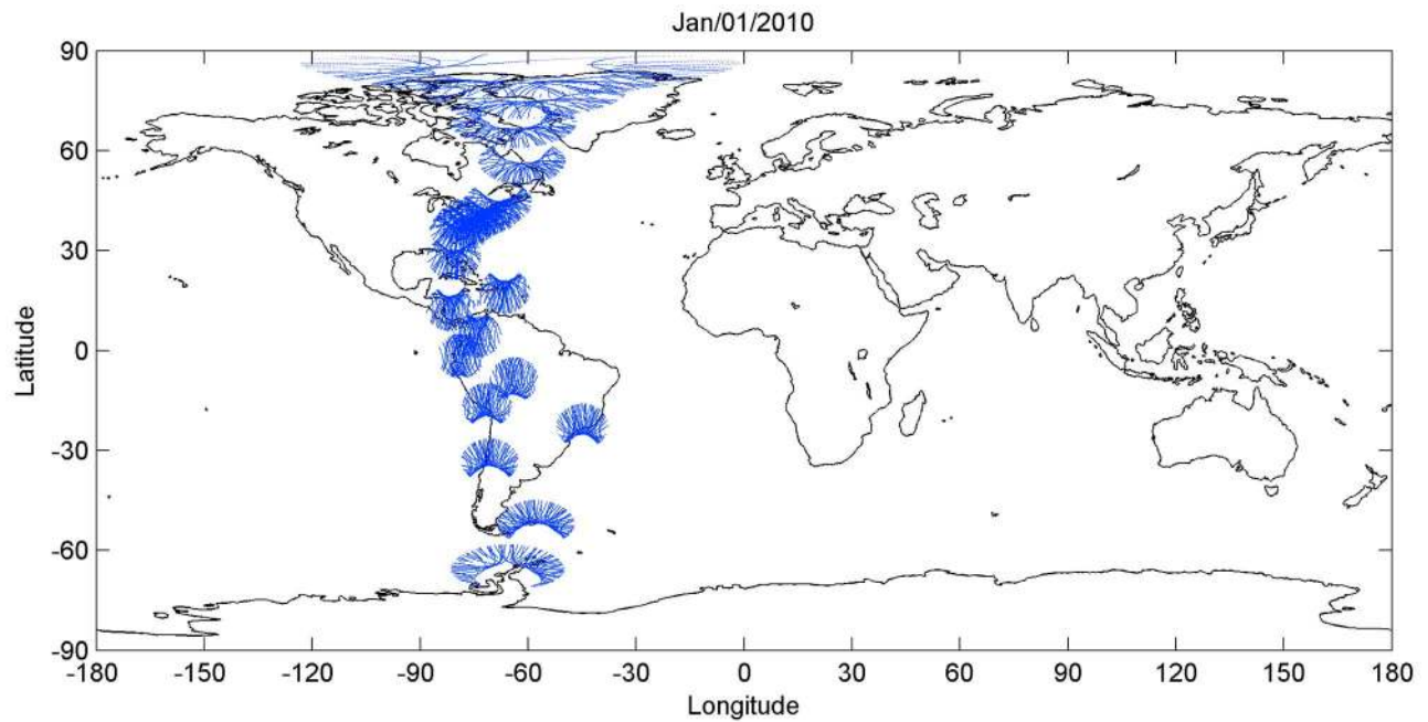
Figure A1. A chain of 21 ground-based GPS receiving stations along the Haiti earthquake longitude 72.5^{\circ}\text{W} is used to produce LTT plots.
