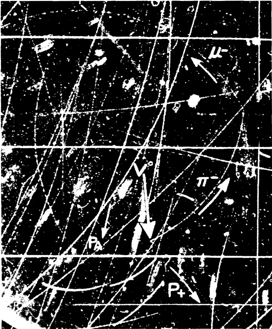
Figure 2. Example of K^0_{L1} \rightarrow \pi^+ + \pi^- neutral particle. P_+ is shown to be a pion by ionization measurements. P_\lambda is a proton track used in the ionization calibration.
