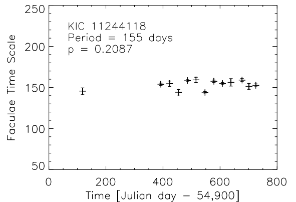
Figure 7. Temporal variability of the facular timescale.
