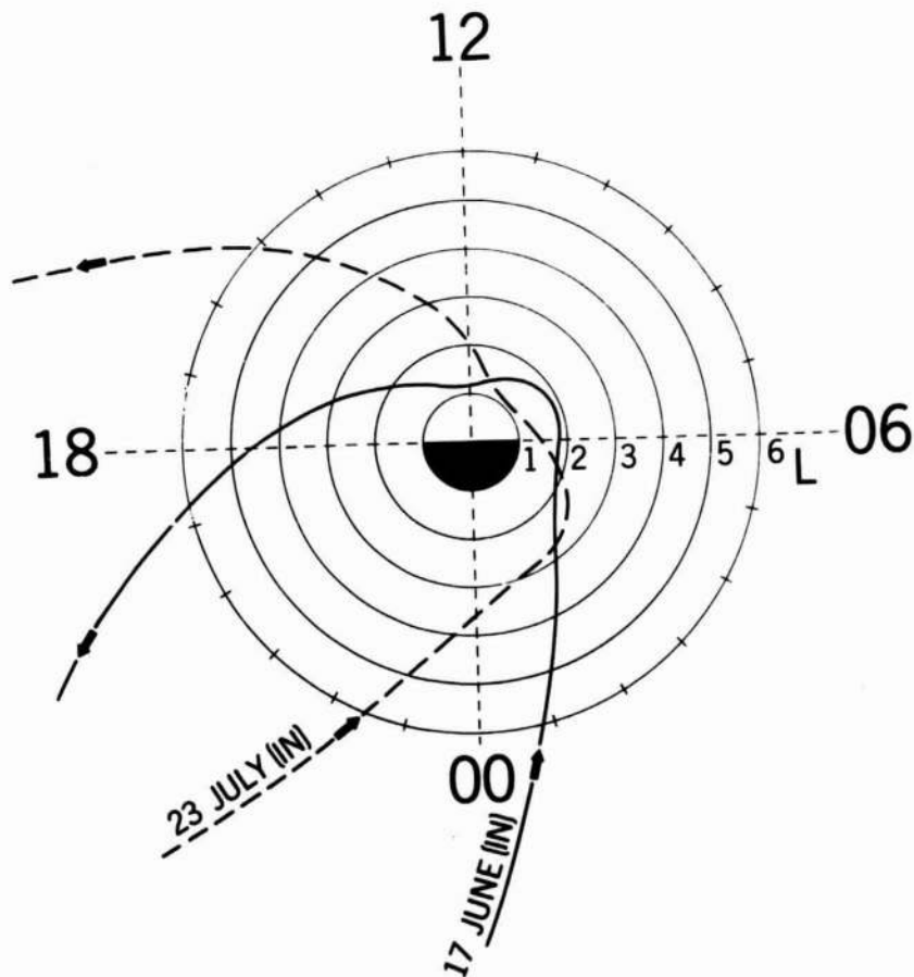
Figure 4—Characteristics of OGJ-3 orbit during June-July 1966. Earth is viewed from above; and displacement between geographic and dipole equatorial planes is neglected. Solid and dashed curves are plots of satellite L and local time position for inbound and outbound arcs. Perigee, 316 km., inclination 31.4^\circ , and period, 48 hr. 35 min.
