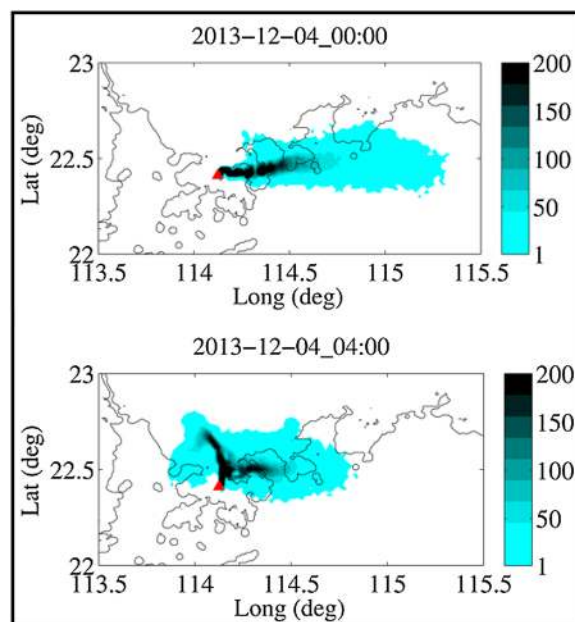
Figure 8. The 12 h backward particle dispersion for 00:00 and 04:00 LT on 4 December 2013. Contours represent the number of particles in each 0.02 latitude \times 0.02 longitude grid.
