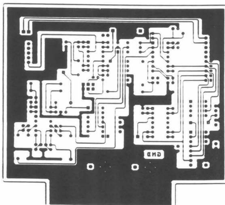
Figure A.10 Printed circuit board layout for the demodulator.
