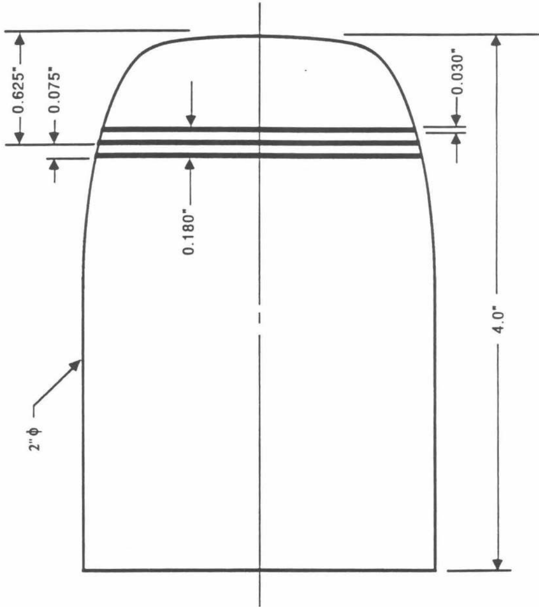
Figure 3.6 Schematic diagram of Schiebe headform with circular electrodes.
