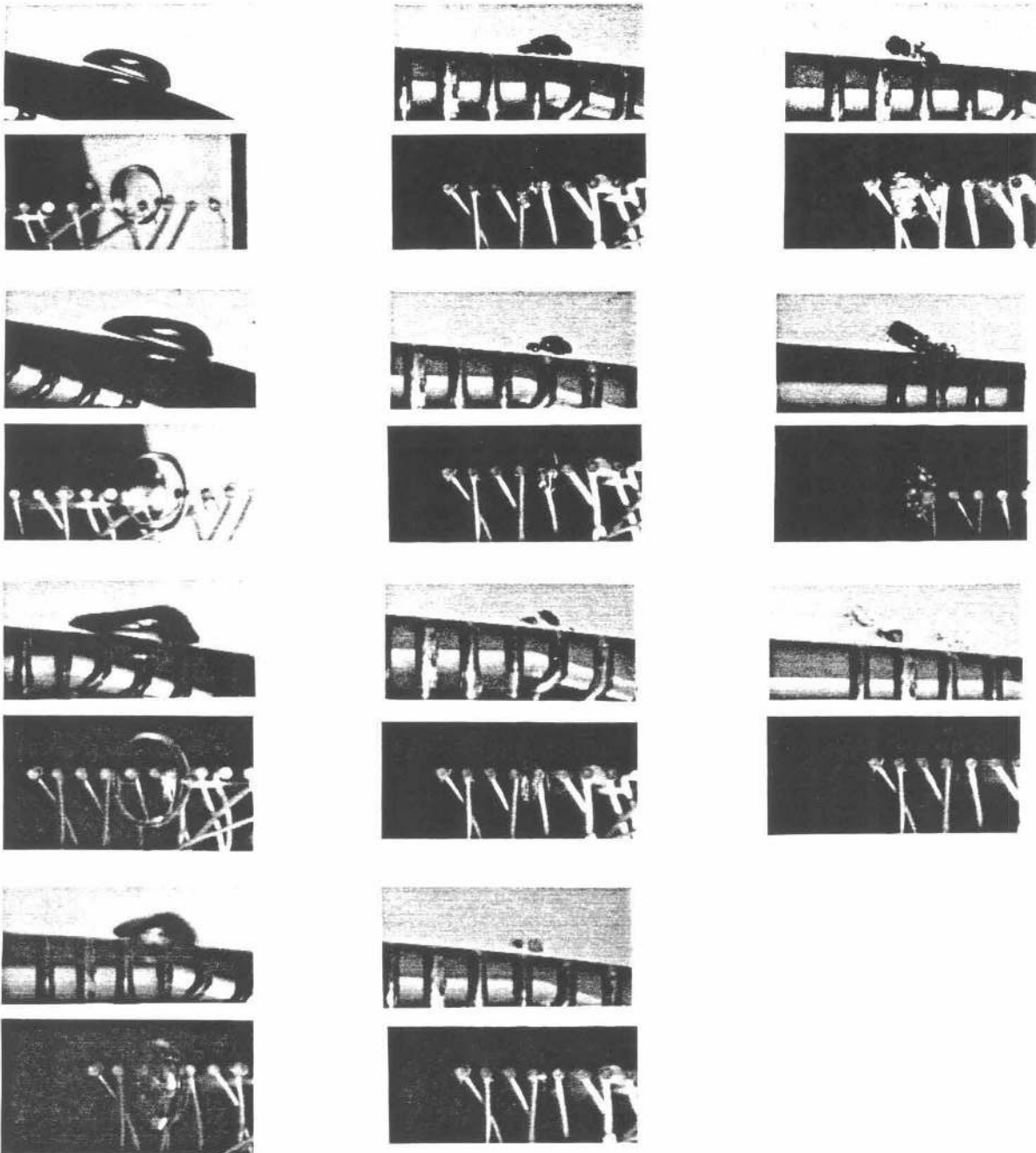
Figure 4.11 Series of photographs detailing typical bubble collapse mechanism on the Schiebe headform, U = 9m/s and \sigma = 0.45 .
