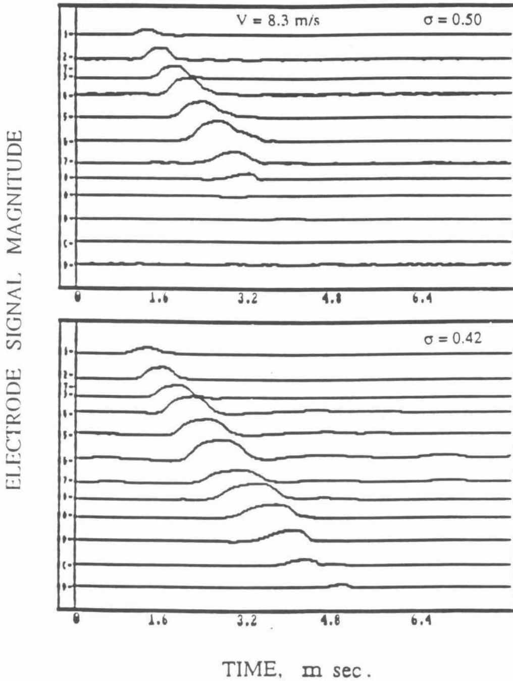
Figure 3.5 Example probe output signal for patch electrodes. Bubbles generated on the I.T.T.C. headform at \sigma = 0.50 and \sigma = 0.42 at U = 8.3\text{m/s} .
