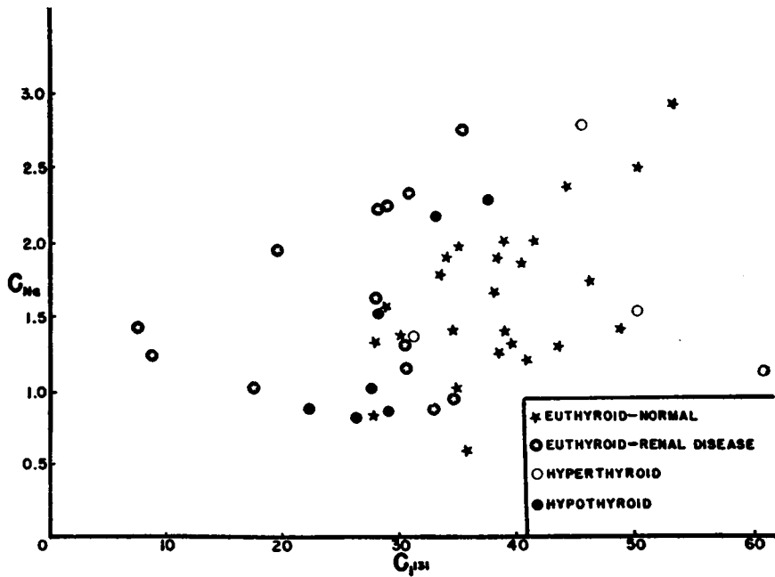
FIG. 5. RELATIONSHIP BETWEEN C_{Na} AND C_{125I}
