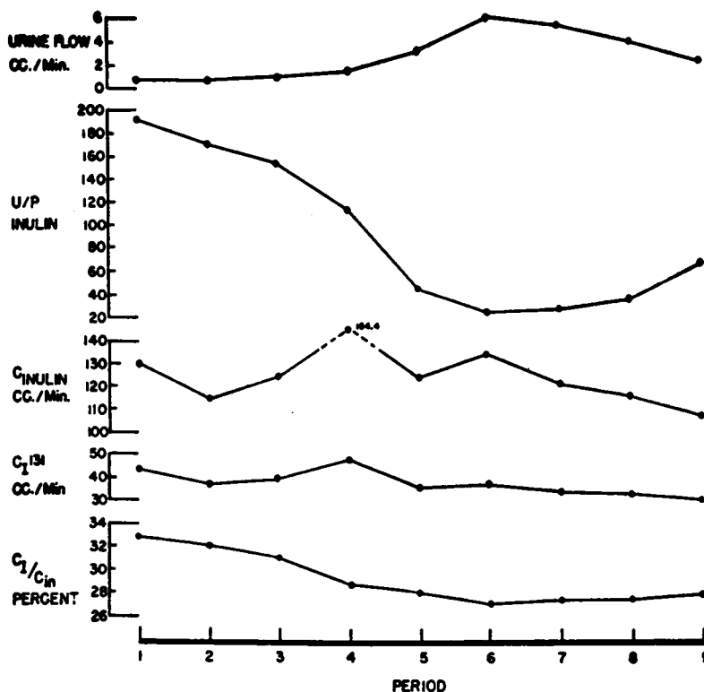
FIG. 9. EFFECTS OF INCREASING URINE FLOW ON C 1 131
