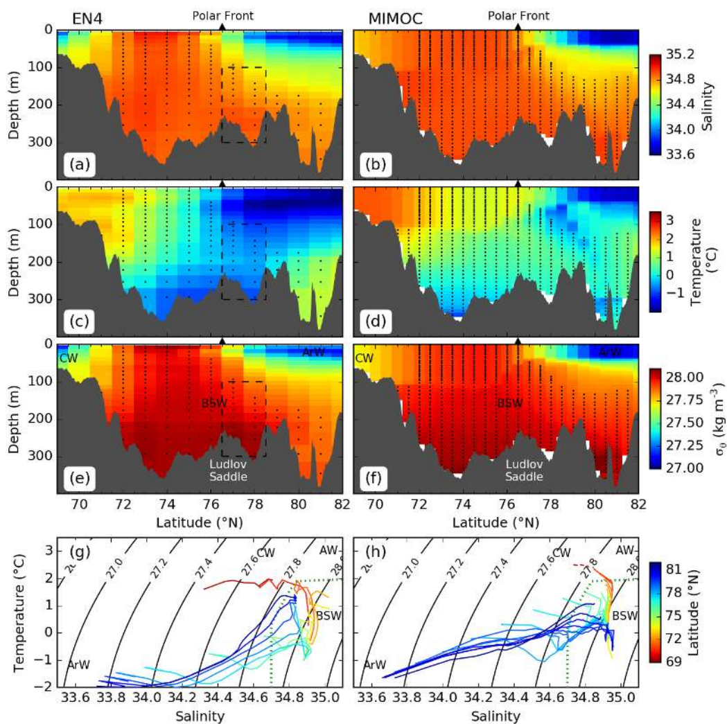
878 FIG. 7. Eastern Barents Sea transect at 44° E (shown in Figure 1) from the MIMOC and EN4 climatology 879 during winter (December, January, February), EN4 is averaged over 1985 – 2016. The Polar Front is marked 880 by the black triangle. (a,b) Salinity, (c,d) temperature and (e,f) potential density. White areas in (a-f) indicate 881 grid cell with no data, black points show the grid cells containing BSW, and the EN4 sub-section (black dashed 882 area) used to produce the BSW temperature and salinities (Figure 6). (g,h) T-S diagrams showing the different 883 water masses present in (a-f). The color indicates the latitude of the profile. The green dotted area in (g,h) 884 shows the limits of the BSW definitions, and AW, ArW and CW water masses are indicated (see Table 1 for their 885 definitions)
