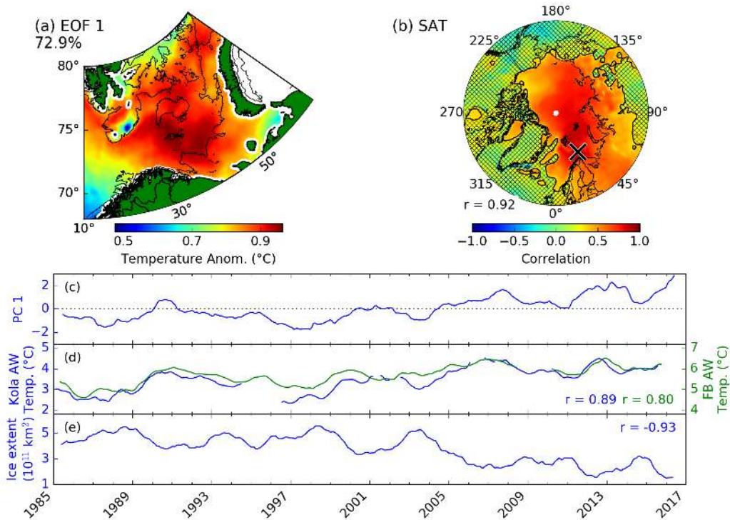
861 FIG. 5. (a) Spatial pattern of first EOF mode of SST variability. The black line indicates the 220 m isobath. 862 (b) Regression of PC 1 with SAT. Maximum correlation (r-value) is shown in the bottom left hand corner and 863 the location of the maximum correlation is shown by a black cross. Hatched areas are not significant at the 864 95%-level. (c) Time series of PC 1. (d) Time series of AW temperature at the Kola section (blue line, 12-month 865 running mean applied) and Fugløya–Bear Island (FB) section (green line, 12-month running mean applied). (e) 866 Time series of sea ice extent in the Barents Sea (12-month running mean applied). Correlations between each 867 variable and PC 1 are indicated.
