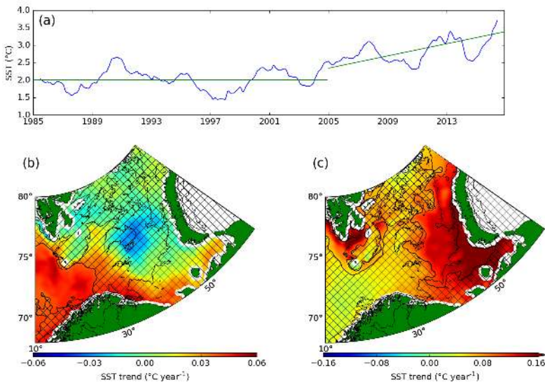
852 FIG. 2. (a) Mean SST across the Barents Sea with a 12-month running mean (blue line). The linear trend for 853 the periods 1985 to 2004 and 2005 to 2016 are shown (green lines). Trend in SST for the periods (b) 1985 to 854 2004 and (c) 2005 to 2016. Note that a different colour scale is used in the two panels. Trends are significant at 855 a level of 95% in un-hatched areas. The black line indicates the 220 m isobath.
