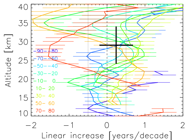
Fig. 11. Vertical profiles of the age of air linear increase/decrease over the years 2002 to 2010 for example latitudes. Horizontal bars give the 2- \sigma uncertainties of the linear variations. The 30-yr trend as derived by Engel et al. (2009) is also shown for comparison as a black cross indicating its valid altitude range and its 2- \sigma uncertainty.
