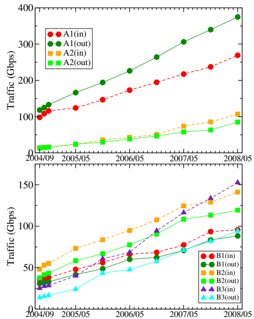
Figure 4: Traffic growth: customer traffic (upper) and external provider traffic (bottom)
