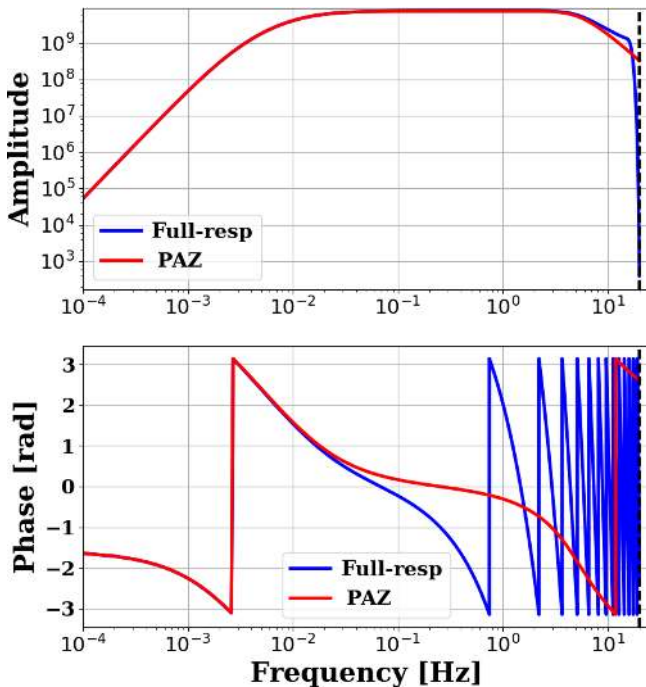
Figure 7. obspsyDMT --plot_stationxml --plotxml_paz --plotxml_min_freq 0.0001 --datapath /path/to/STXML.GT.LBTB.00.BHZ Transfer function spectra (amplitude and phase) of a Geotech KS-54000 borehole seismometer (GT.LBTB) in Botswana. Blue lines show transfer function components computed for all filter stages in the StationXML file; red lines are for the analog part. A large discrepancy exists between the phase spectra of the two transfer functions. The deviation emerges at frequencies around 10^{-2} Hz and increases up to the Nyquist frequency. Fig. 8 shows that this difference is caused by one of the digital stages in the instrument response.
