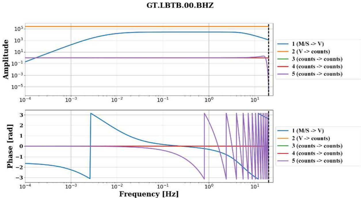
Figure 8. obspsyDMT --datapath /path/to/STXML.GT.LBTB.00.BHZ --plot_stationxml --plotxml_min_freq 0.0001 --plotxml_allstages Transfer function spectra (amplitude and phase) of each stage in the StationXML file of a Geotech KS-54000 borehole seismometer (GT.LBTB) in Botswana. In the phase response, two stages (1 and 5) have non-zero values. Both stages contribute to the phase spectrum of the complete instrument response (“full-resp”) of Fig. 7. However, the effects of Stage 5 on amplitude and phase spectra are not considered in PAZ (analog).
