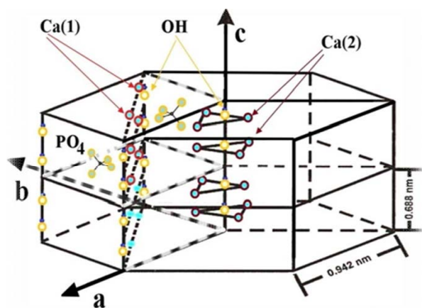
Fig. 3. Elementary cell of HAP [15] and EDX of HAP.
