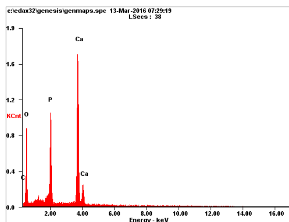
Fig. 3. Elementary cell of HAP [15] and EDX of HAP.
