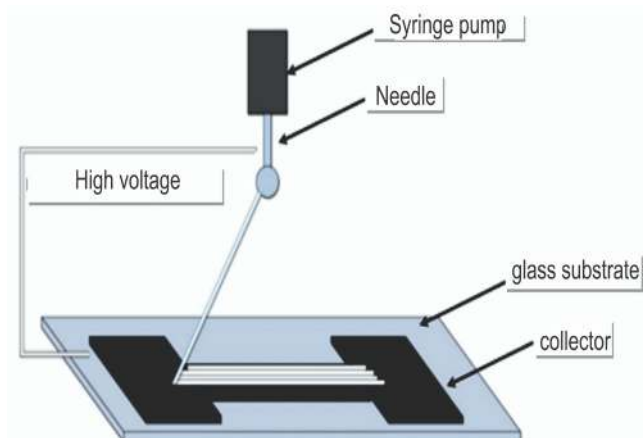
Fig. 4. Schematic representation of the experimental setup.
