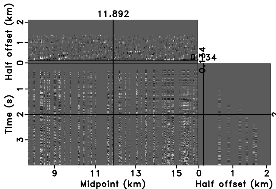
Figure 16: Marine data with 70% traces removed.
