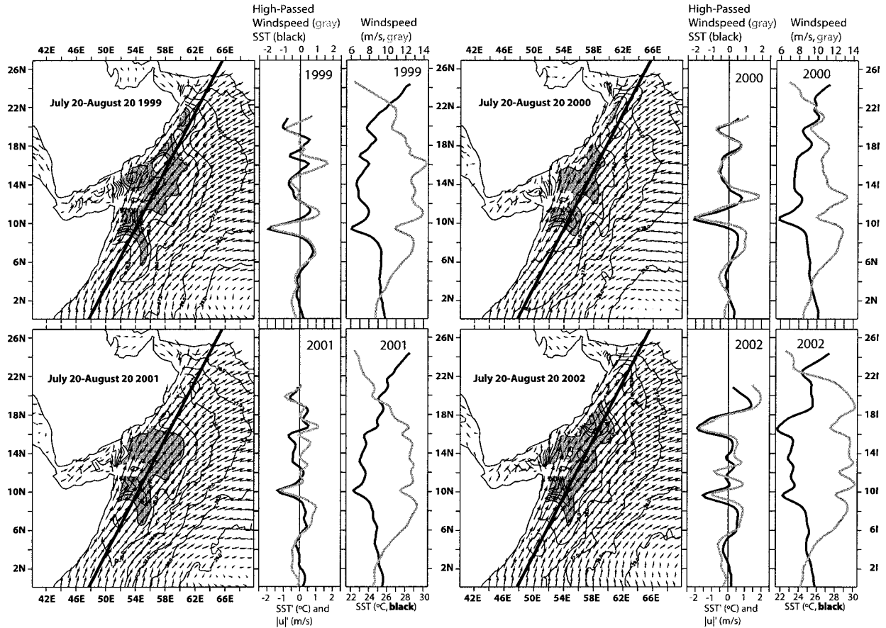
FIG. 4. Structure of “along-wind” SST from TMI and wind speed from QuickScat, and high-pass filtered SST from TMI and QuickScat averaged 20 Jul–20 Aug for each year 1999–2002. Shown for each year is an x - y map of the averaged SST and wind velocity, and the track along which the data are sampled. The meridional sections show, for each year, the high-pass-filtered and total wind and SST ( ^{\circ}\text{C} ) sampled along the track.
