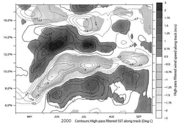
FIG. 5. Time evolution of along-wind high-pass-filtered SST (contoured, ^{\circ}\text{C} ), wind speed (shaded, \text{m s}^{-1} ) during the southwest monsoon of 2000. Evolution computed along the track shown in Fig. 4. Both fields are 15-day boxcar smoothed in time.
