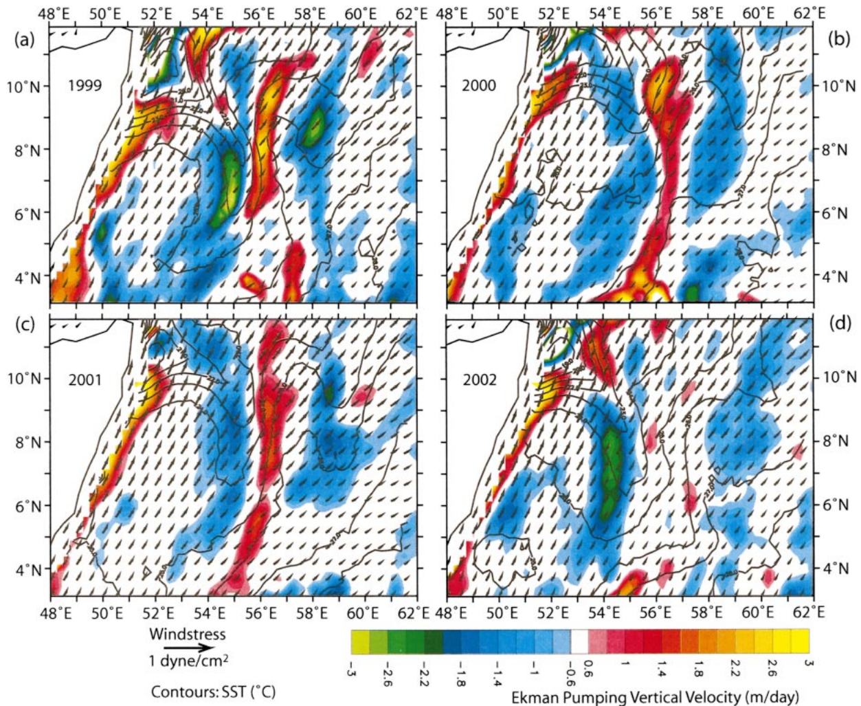
FIG. 3. Maps of SST (contour) and vertical Ekman pumping velocity (shading) over the “Great Whirl” region, averaged 20 Jul–20 Aug for (a) 1999, (b) 2000, (c) 2001, and (d) 2002. SST is from TMI, units are ^{\circ}\text{C} with a contour interval of 1^{\circ}\text{C} . Vertical Ekman pumping velocity is computed from QuickScat winds, units are \text{m day}^{-1} , positive is upwards.
