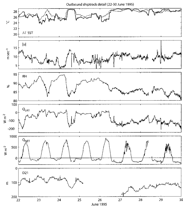
FIG. 8. (top) Outbound leg along-track observations of air temperature and sea surface temperature (AT and SST); wind speed ( |u| ), relative humidity (RH), specific humidity ( q ), the latent heat flux ( Q_{LAT} ), the net surface heat flux ( Q_{NET} ) and 24-hr running average, and the depth of the 21°C isotherm from the SeaSoar data (D21). Over cold water, there is a reduction in the wind speed and a near saturation of the RH, both contributing to the sharp drop in the latent heat loss. The jump in the AT – SST difference over cold SSTs suggests that the near-surface atmosphere has stratified. The colder SSTs are associated with a thermocline that is closer to the surface.
