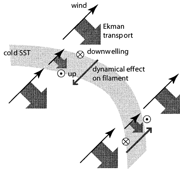
FIG. 9. Schematic of cold filaments and wind curl. Upwelling and downwelling Ekman pumping anomalies are dependent on the orientation of the filament to the mean wind direction.
