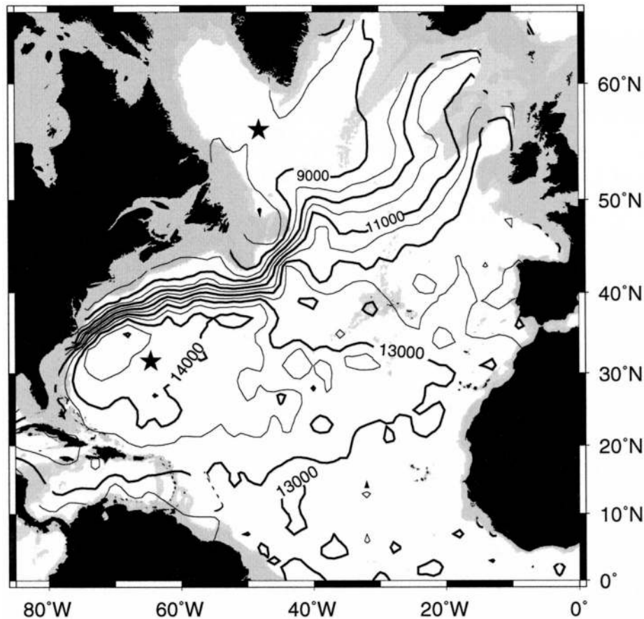
FIG. 2. Climatological mean field of potential energy anomaly (PEA) at the sea surface relative to 2000 db. Contour interval is 500 \text{ ergs cm}^{-2} . Stars indicate the locations of time series data in the Labrador Basin and near Bermuda used to construct the transport index in Fig. 1.
