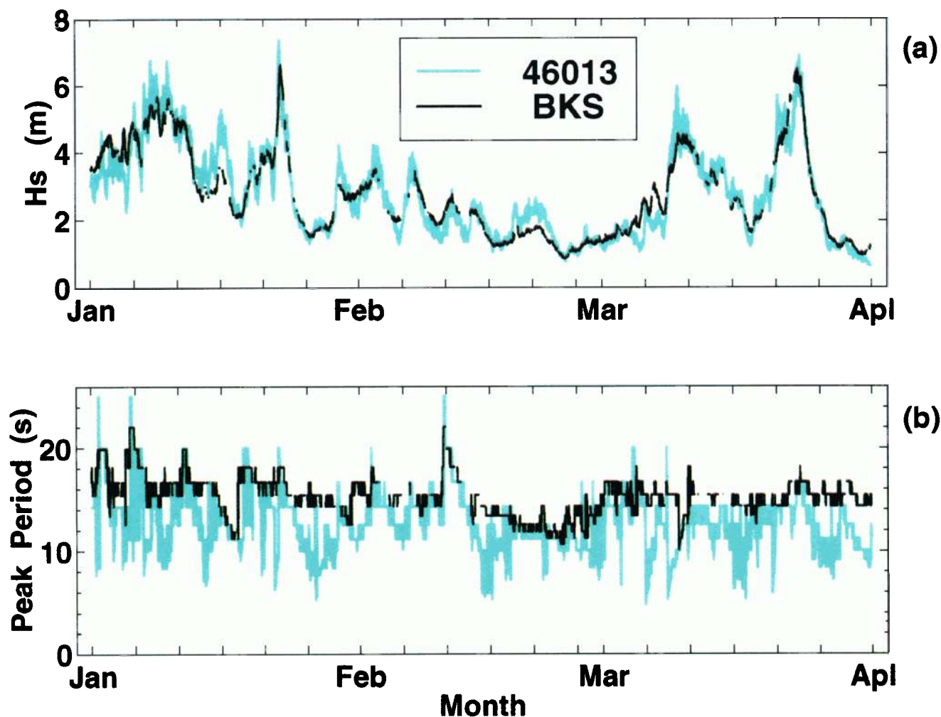
Plate 3. (a) Significant wave height H_s at NOAA buoy 46013 for January-March 1995 (blue line) and the seismic reconstruction (black line) from BKS ( \hat{H}_s ) for the same time period. (b) Associated peak wave period T_p at 46026 and the corresponding reconstruction \hat{T}_p from BKS.
