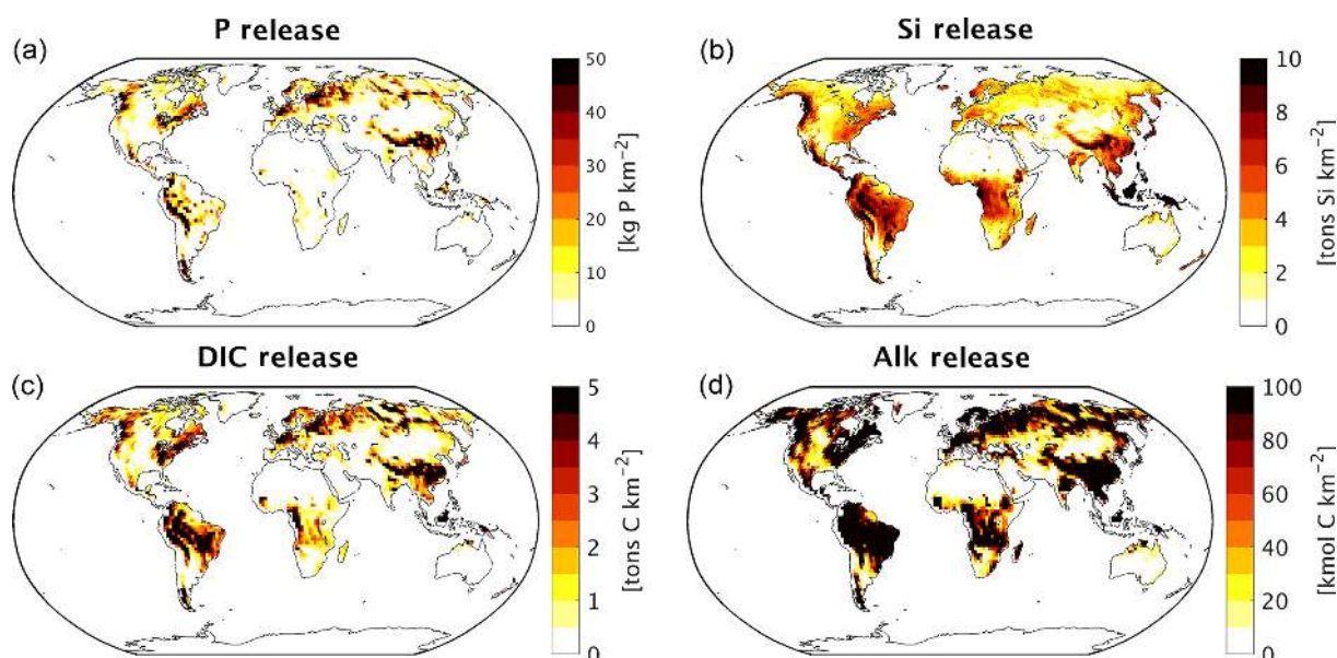
Figure 2. Weathering release yields of (a) P ( \text{kg P km}^{-2} ), (b) Si ( \text{t Si km}^{-2} ) and (c) DIC ( \text{t C km}^{-2} ).
