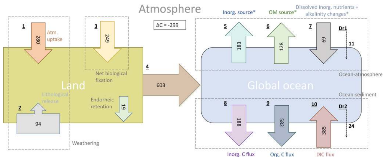
Figure 9. Origins and oceanic fate of riverine C in our framework ( \text{Tg C yr}^{-1} ). (1) Atmospheric C uptake through weathering. (2) Carbonate weathering C flux from the lithology. (3) Net land biological C uptake (derived directly from riverine organic C exports). (4) Total riverine C exports. (5) Oceanic C outgassing from riverine DIC (i.e., inorganic C) inputs. (6) Oceanic C outgassing resulting from riverine tDOM inputs. (7) Oceanic C uptake due to the enhanced primary production by dissolved inorganic nutrients and the corresponding alkalinity production. (8) Simulated inorganic C deposition (i.e., \text{CaCO}_3 to the sediment). (9) Simulated net organic C (i.e., POM) deposition to sediment. (10) Diffusive DIC flux from the sediment pore water back to the water column. Given are simulated fluxes by the terrestrial and ocean models, except when * is stated, meaning that the fluxes were calculated assuming model equilibrium. Dr1 and Dr2 are the calculated drifts between the simulated oceanic C fluxes and the calculated equilibrium fluxes (derived from model equations, Appendix C2) for the ocean–atmosphere and ocean–sediment interfaces, respectively. See Appendix C for the calculation of all fluxes.
