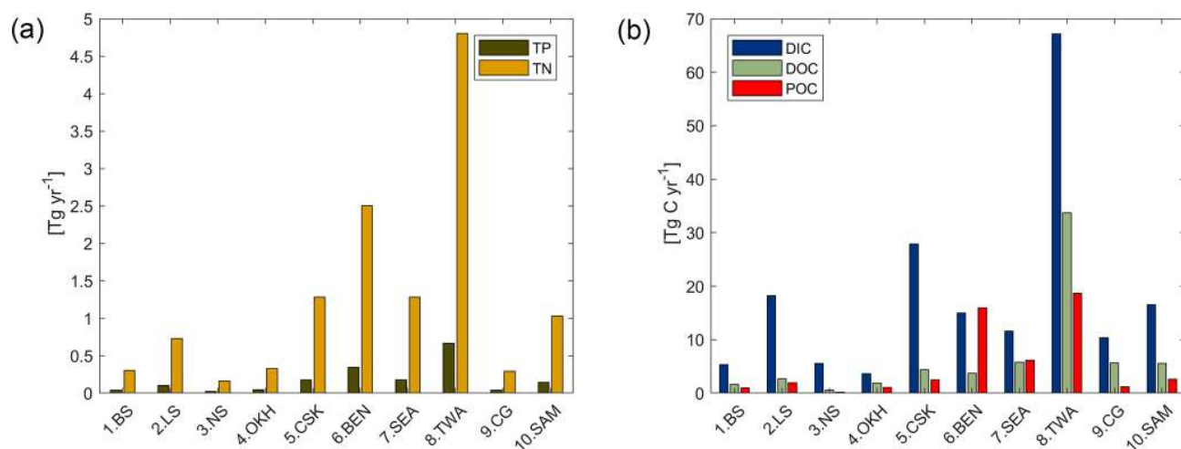
Figure 7. Modeled riverine (a) P (TP) and N (TN), and (b) C (DIC, DOC and POC) exports to selected coastal regions. TP and TN are the total P and N from the sum of their riverine dissolved inorganic loads (DIP, DIN) and of their riverine organic loads (P and N within tDOM and POM). DOC and POC are the C loads within riverine tDOM and POM, respectively.
