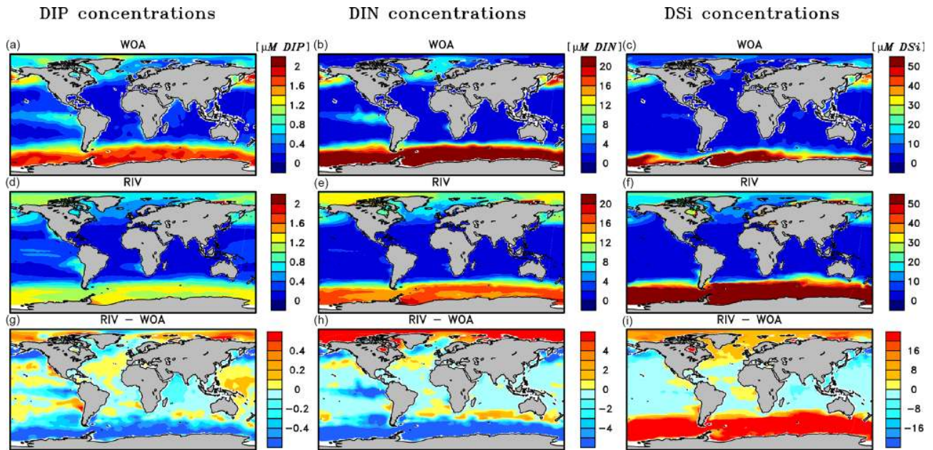
Figure 4. Surface DIP (a, d, g), DIN (b, e, h) and DSi (c, f, i) concentrations in WOA observations (a, b, c), RIV (d, e, f) and their differences RIV-WOA (g, h, i).
