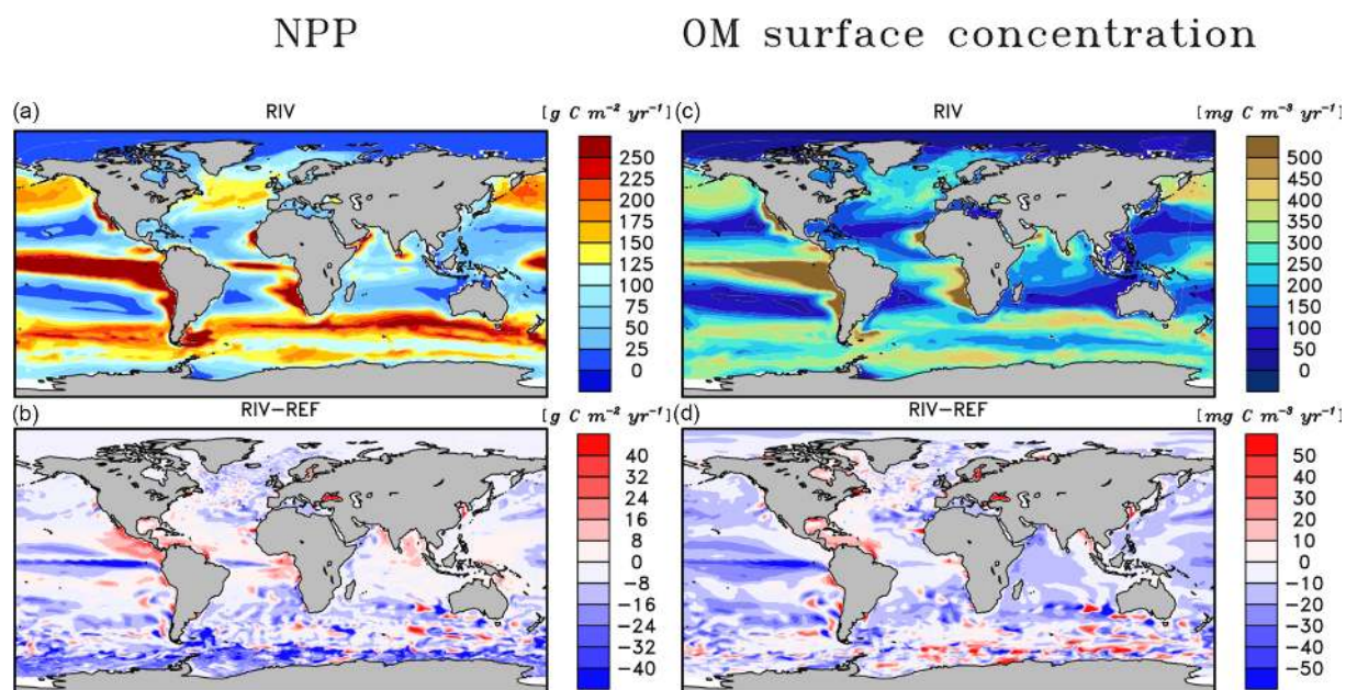
Figure 5. Depth integrated annual NPP (a, b) and total annually accumulated organic matter concentration (c, d) in the surface layer in the RIV simulation and RIV - REF.
