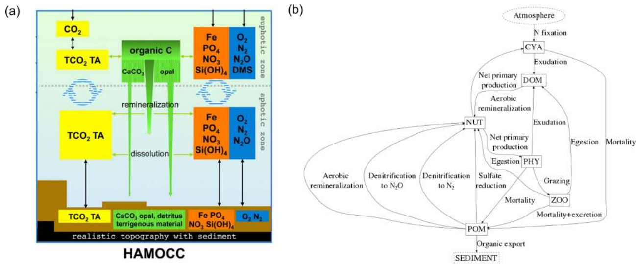
Figure A1. (a) Scheme of model compartments in HAMOCC, modified from Ilyina et al. (2013) and (b) scheme of the organic dynamics taking place in the model. The most central model parameters can be found in the Supplement S2.
