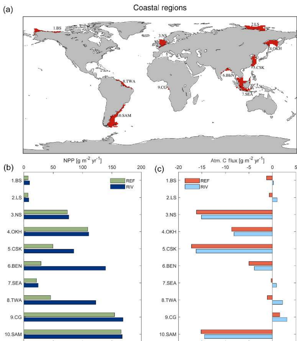
Figure 8. (a) Global map of the 10 chosen coastal regions with depths of less than 250 m, (b) pre-industrial annual NPP per area and (c) CO 2 flux in the given regions ( \text{g C m}^{-2} \text{yr}^{-1} ). In (c), a positive flux means a flux from the ocean to the atmosphere.
