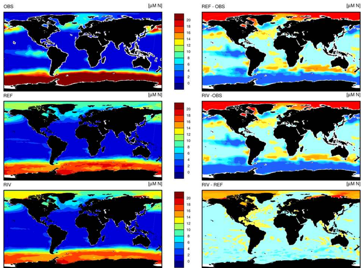
Figure D3. Nitrate (DIN) concentrations in OBS (WOA observations), REF and RIV.
