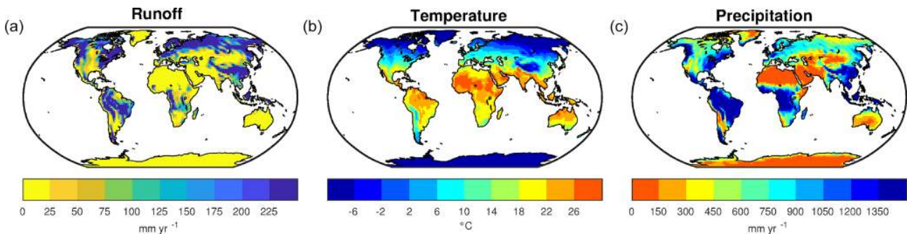
Figure B1. Modeled pre-industrial (a) surface runoff ( \text{mm a}^{-1} ), (b) surface temperature ( ^{\circ}\text{C} ) and (c) precipitation ( \text{mm a}^{-1} ) annual means.
