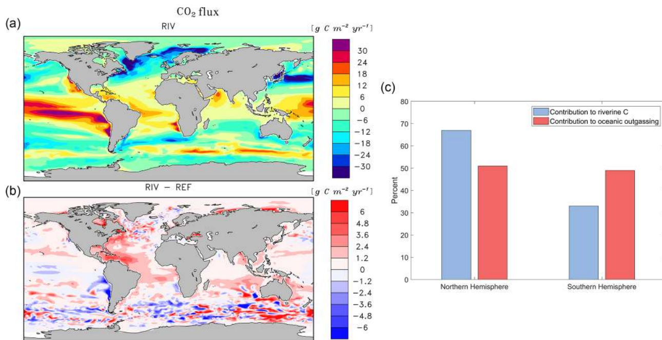
Figure 6. Annual pre-industrial air-sea CO 2 flux of (a) RIV, (b) RIV-REF, and (c) contributions of the Northern Hemisphere and Southern Hemisphere to riverine C loads and oceanic riverine C outgassing. A positive flux in (a) and (b) describes an outgassing flux from the ocean to the atmosphere, whereas a negative flux is a flux from the atmosphere to the ocean.
