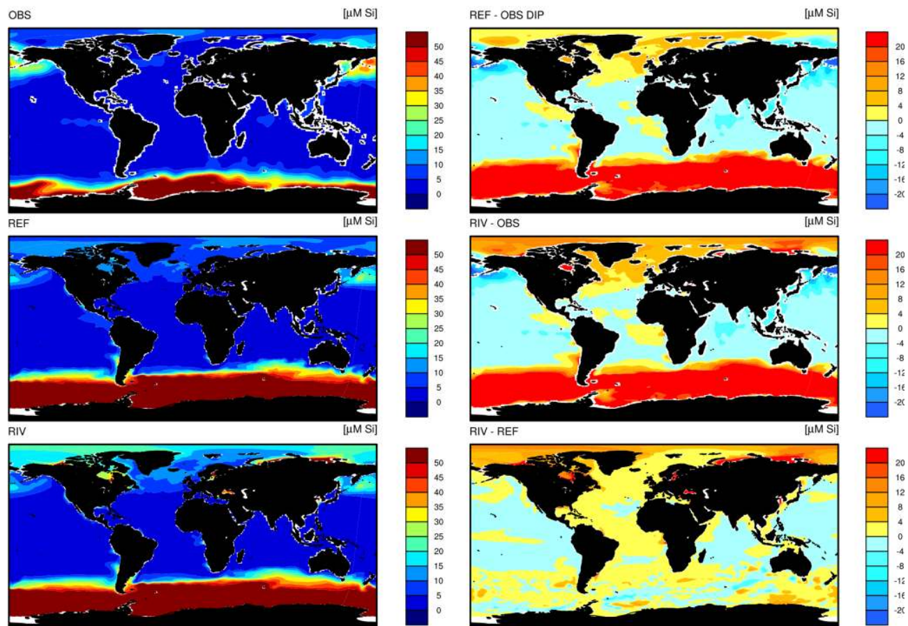
Figure D2. Dissolved silica (DSi) concentrations in OBS (WOA observations), REF and RIV.
