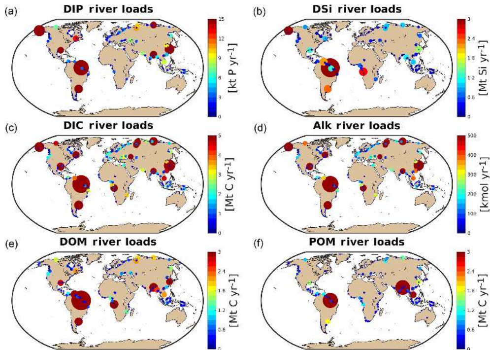
Figure 3. Modeled annual river loads of DIP (a), DSi (b), DIC (c), Alk (d), DOM (e) and POM (f).
