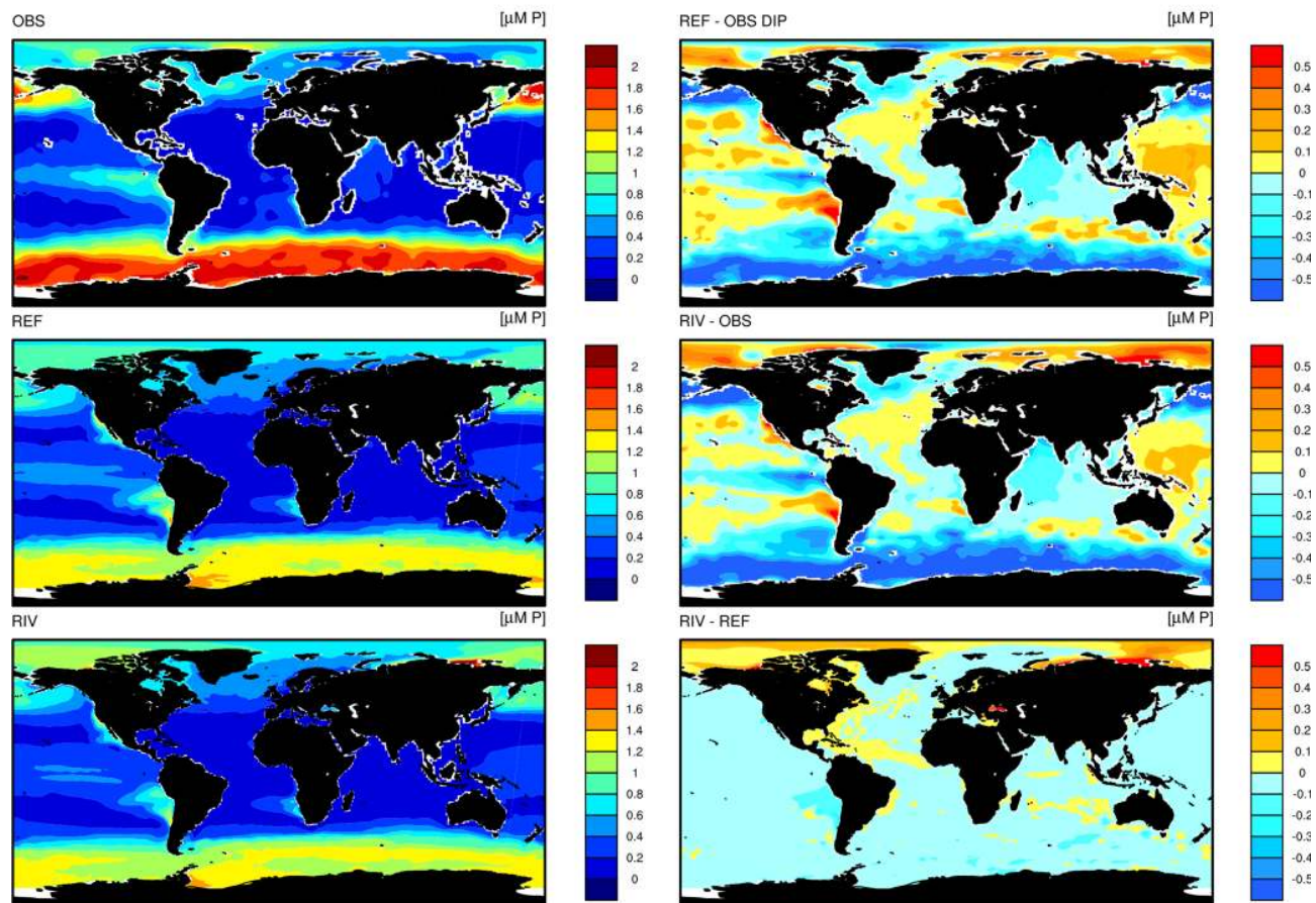
Figure D1. DIP concentrations in OBS (WOA observations), REF and RIV.
