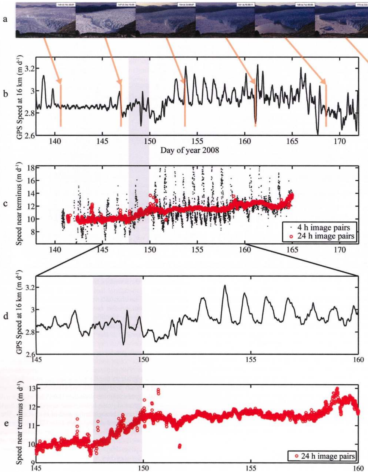
Fig. 2. (a) A set of time-lapse images taken at \sim 7 day intervals showing the evolution of the terminus region. (b, c) The corresponding ice-speed records from (b) the on-ice GPS station, \sim 16 km from the terminus, and (c) photogrammetry, near the terminus. The gray shaded region indicates break-up of the ice melange, as observed in the time-lapse images. (d, e) The period between days 145 and 160 is emphasized for (d) the on-ice GPS and (e) the near-terminus region.
