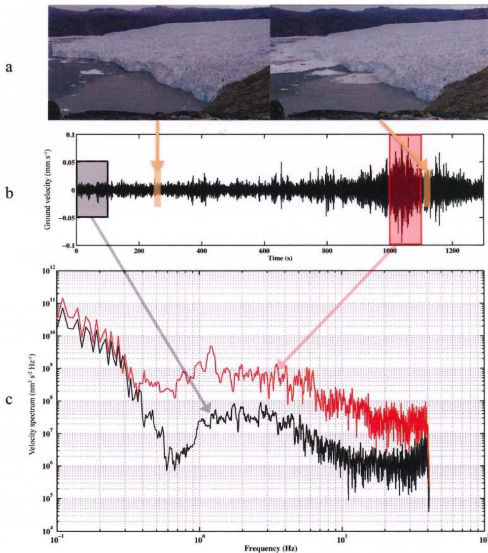
Fig. 5. (a) Pair of time-lapse photos indicating a calving event occurring in the left third of the frame. (b) The east component seismic record from a station co-located with the time-lapse camera. We compute spectra for windows of 100 s during two periods, shown as signal and noise. (c) The spectra indicate increased energy above noise levels from \sim 0.3 Hz to the Nyquist frequency.
