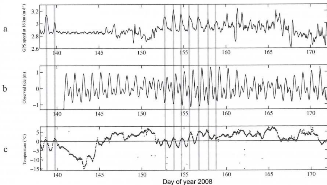
Fig. 4. Measurements during days 140–170 of (a) ice flow speed, from the on-ice GPS stations ~16 km from the terminus, (b) measured tide in the fjord and (c) air temperature measured at an AWS co-located with the GPS station.
