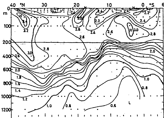
Figure 2. Methane concentration section from 40^\circ \text{ N} to 5^\circ \text{ S} along 165^\circ \text{ E} . Contour interval is 0.2 \text{ nM} . The mixed layer methane maximum is evident in this section. Reprinted from ref 84, Copyright 1995, with kind permission of Springer Science and Business Media.
