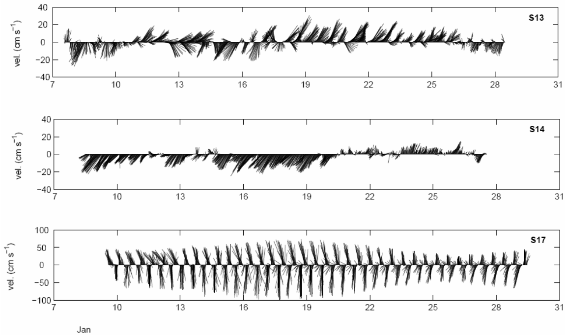
Figure 9 – Time series of the current vectors at stations 13 (top), 14 (middle) and 17 (bottom) during the summer and according to the location map presented in Figure 2. The vectors are related to the true north.
