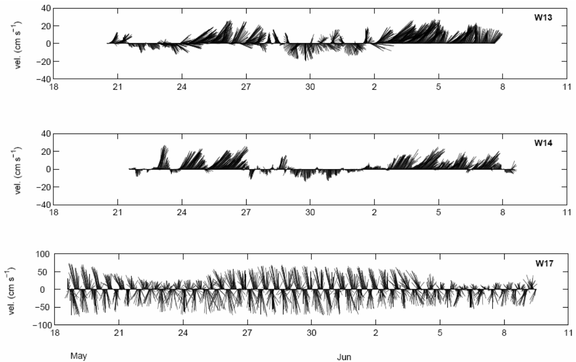
Figure 10 – Same as Figure 9, but for the winter.
