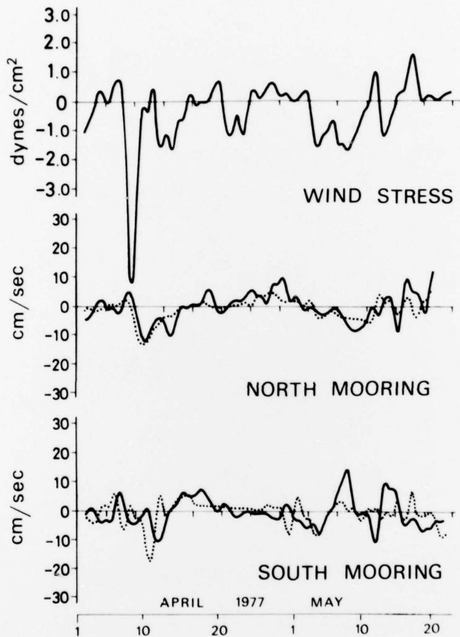
FIG. 8 TIME SERIES OF THE LOWPASS COMPONENTS OF WIND STRESS AND COASTAL CURRENTS. The currents at 20 m are shown by solid curves, those at 80 m are shown by dotted curves.
