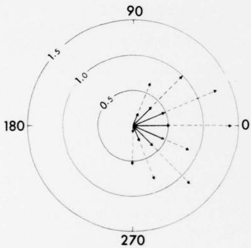
FIG. 6 DIRECTIONAL STATISTICS OF THE LARGE-SCALE MEAN WIND STRESS. The solid arrows represent the mean components and the dashed arrows show the standard deviations; units are dynes/cm 2 .
