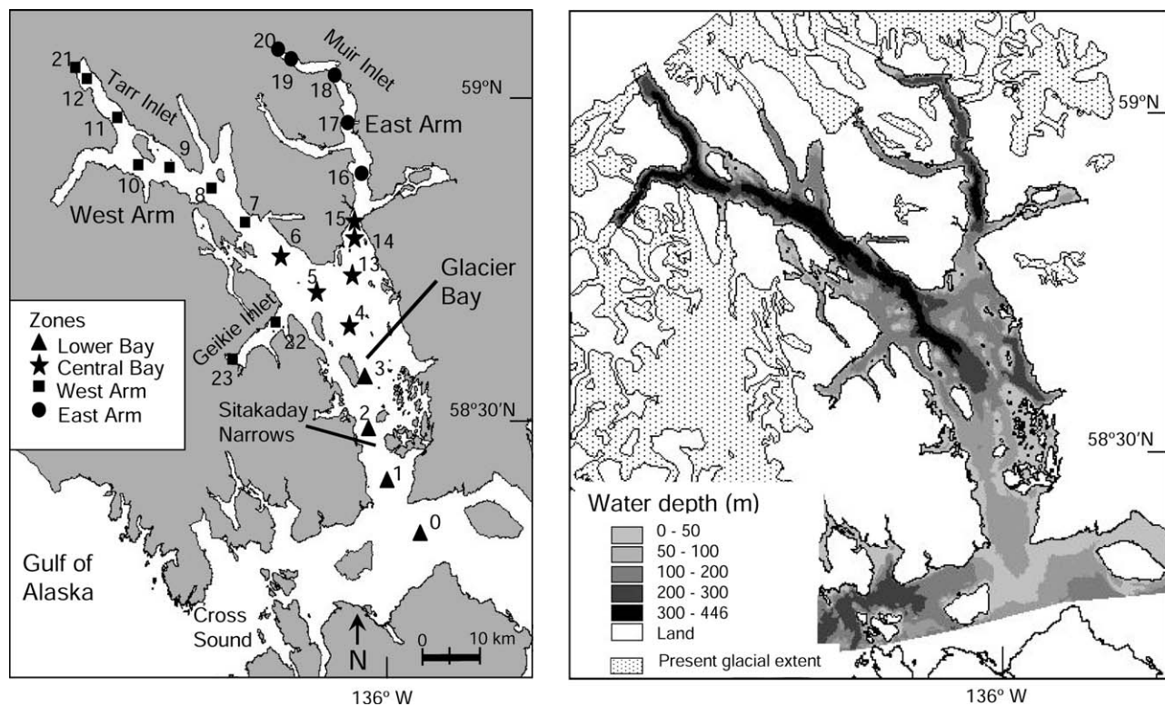
Fig. 1. Glacier Bay, Alaska, USA and the oceanographic sampling stations. Stations were grouped into four zones based on physical properties such as similarities in bathymetry, relative position to glaciers and source of oceanic waters, and general examination of oceanographic patterns. Zones were defined as lower Bay (stations 0, 1, 2, 3), central Bay (stations 4, 5, 6, 13, 14, 15), West Arm (stations 7, 8, 9, 10, 11, 12, 21, 22, 23), and East Arm (stations 16, 17, 18, 19, 20). Plan view of Glacier Bay bathymetry and location of present glacial extent. Gray and black shadings represent deeper portions of the Bay, while light gray shading represents shallower depths.
