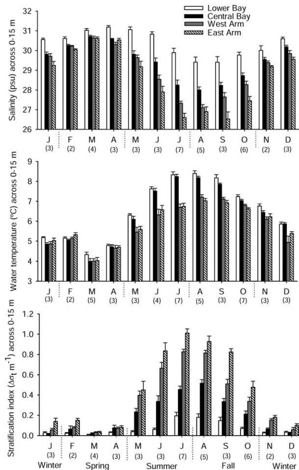
Fig. 5. Oceanographic patterns as a function of month and zone. Values represent means (+ standard error) of each of the parameters from all casts averaged over the top 15 m of the water column across each month for each zone: Salinity, water temperature, and stratification. Season definitions used in analyses are illustrated. The number of years for which data were obtained is indicated in parentheses below each month; numerous casts were taken within each zone during each sampling trip.
