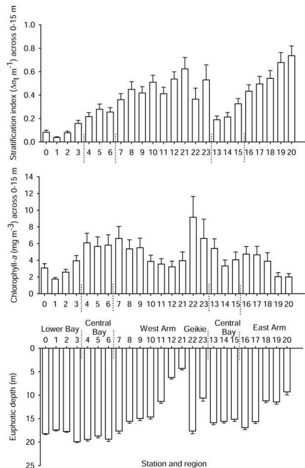
Fig. 7. Oceanographic patterns by station within Glacier Bay. Values represent means (+ standard error) of each of the parameters from all casts and averaged across each station: stratification, chlorophyll a , and euphotic depth. Zones (as defined for analyses) are indicated below the station numbers. Stations are oriented from the mouth to the head of the Bay, with stations 0–12 and 21 representing the axis of the Bay from Icy Strait to the head of Tarr Inlet (West Arm), stations 22 and 23 characterizing Geikie Inlet, and stations 13–20 representing the Muir Inlet (East Arm) axis. The euphotic depth is defined here as the depth at which the amount of light (photosynthetically available radiation – PAR) measured is 1% of that at the surface.
