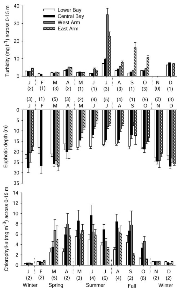
Fig. 6. Oceanographic patterns by month and zone. Values represent means (+ standard error) of each of the parameters from all casts averaged over the top 15 m of the water column across each month for each zone: turbidity (optical backscatterance), euphotic depth, and chlorophyll a . The euphotic depth is defined here as the depth at which the amount of light (photosynthetically available radiation – PAR) measured is 1% of that at the surface. The number of years for which data were obtained is indicated in parentheses below each month; numerous casts were taken within each zone during each sampling trip.
