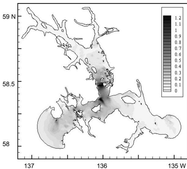
Fig. 4. Grayscale contours of root-mean-square (RMS) values of tidal current speed ( \text{m s}^{-1} ) for the Glacier Bay domain. Results are obtained from the harmonic analysis of ADCIRC simulations of tidal circulation in the Bay.
