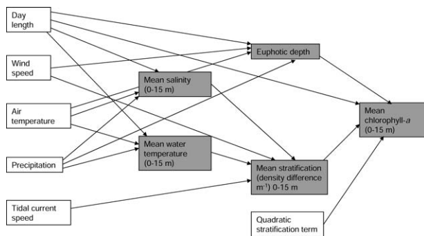
Fig. 3. Hypothesized relationships between external physical factors, oceanographic parameters, and chlorophyll a within Glacier Bay, Alaska. The response variables for the five separate multiple regression models are shaded in gray. The arrows connect explanatory variables to response variables, and illustrate all potential causative parameters that were included in the multiple regression selection procedure to determine the best-fit model describing the response variable.
