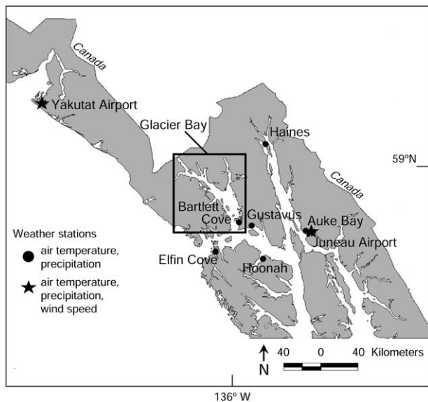
Fig. 2. Weather stations in the vicinity of Glacier Bay, Alaska. Data from the eight weather stations were averaged to obtain regional patterns of air temperature and precipitation. Data from the Juneau Airport and Yakutat Airport stations were averaged to obtain regional patterns of wind speed.
