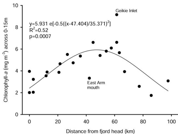
Fig. 8. Relationship between the distance from the head of the fjord and chlorophyll a abundance. Chlorophyll a values represent averages over the top 15 m of the water column pooled over all sampling periods for each station. Each data point represents the value for one station. Results from nonlinear regression analyses are presented. The data point that lies far above the model fit at approximately 65 km represents station 22 (high chlorophyll a values in Geikie Inlet), and the data point below the model fit at approximately 40 km is the value for station 14 (situated at the East Arm sill in shallower, less-stratified water).
