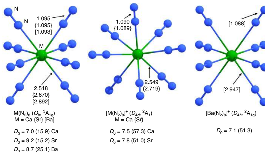
Fig. 2 Calculated geometries and bond lengths. Calculated equilibrium structures and interatomic distances [ \text{\AA} ] of M(N_2)_8 and [M(N_2)_8]^+ ( M = \text{Ca}, \text{Sr}, \text{Ba} ) at the M06-2X-D3/def2-TZVPP level. Bond dissociation energies D_0 [ \text{kcal mol}^{-1} ] for loss of one N_2 and (in parentheses) loss of eight N_2
