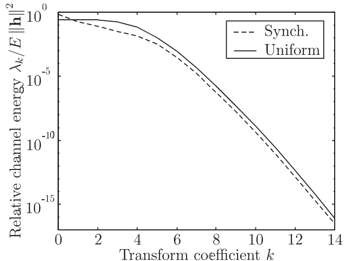
Fig. 4. Relative channel energy in the transform coefficients for the two channels addressed.
