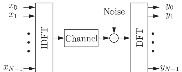
Fig. 1. Base band model of an OFDM system. A cyclic prefix is used, but not displayed here.
