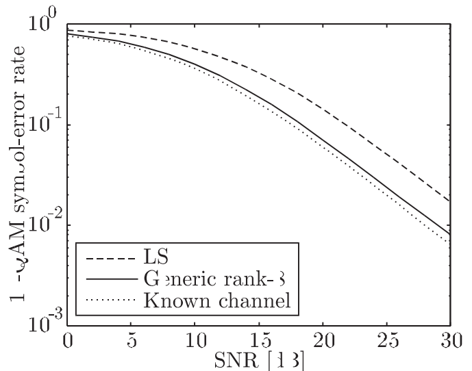
Fig. 7. SER for 16-QAM training data and a synchronized channel. Generic rank-8 estimator, designed for a uniform channel and 30 dB in SNR, is compared to two references: The LS estimator and known channel at the receiver.
