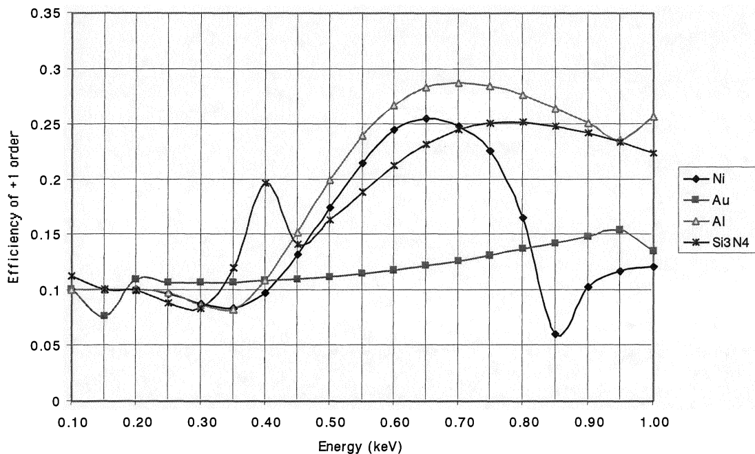
Figure 4. Calculated efficiencies of Ni, Au, Al and silicon nitride as a function of photon energy for a thin zone plate
