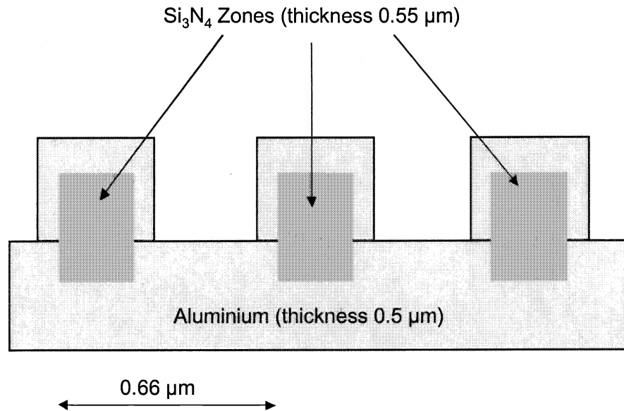
Figure 3. Mechanical layout of the zone plate to be manufactured by the following steps (1) coat one side of a 0.55 μm thick silicon nitride window with aluminum, (2) e-beam write and etch the zone-plate pattern into the silicon nitride material and (3) coat the other side of the window with aluminum such that the total vertical thickness of aluminum is 0.5 μm.
