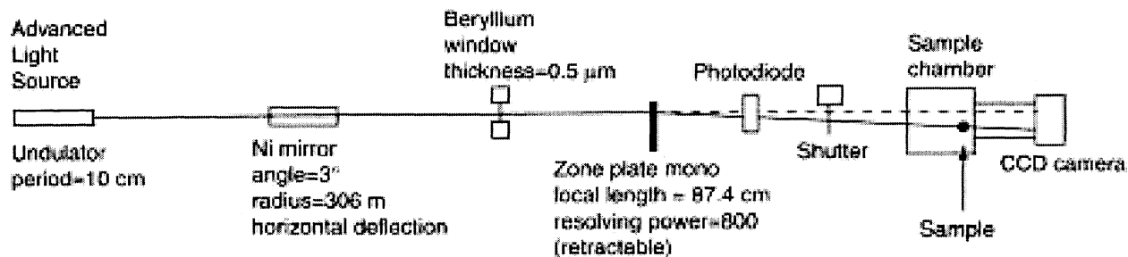
Fig. 1. Beam line overview from the side
