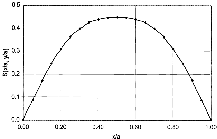
Fig. 7. Universal function describing the temperature distribution over an x-ray-heated square window. The plot is taken along the line y=a/2
