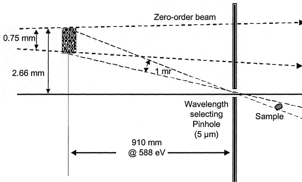
Figure 2. General monochromator layout
