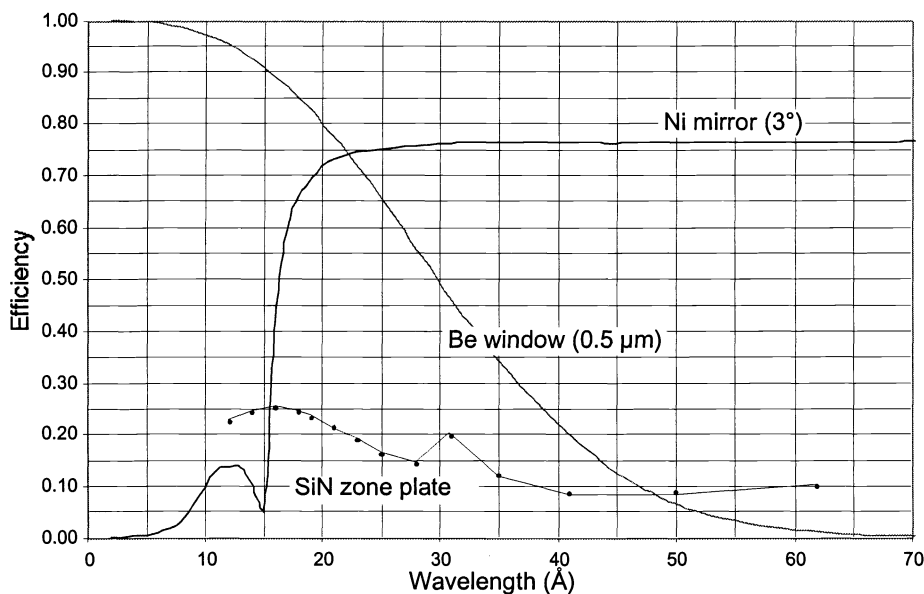
Fig. 5. X-ray efficiencies of the mirror (3° nickel), window (0.5 μm beryllium) and zone plate (0.55 μm silicon nitride)
