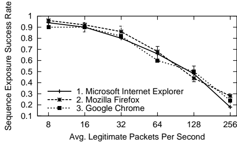
Figure 4: TCP sequence exposure success rate. Each measurement is the average of 50 runs, error bars mark standard deviations.
