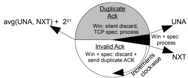
Figure 3: Ack Number Map. UNA is the lowest unacknowledged sequence number, NXT is the next sequence number that C will send. The 32-bit Ack field is cyclic.
