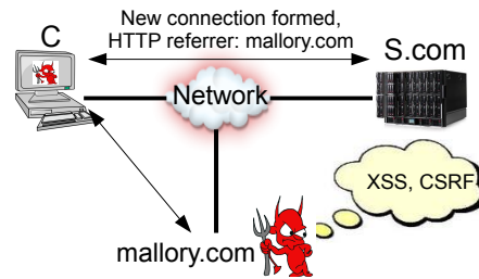
Figure 1: Network Model. C enters www.mallory.com , the adversarial web page. A script on that page forms a connection with www.s.com .
