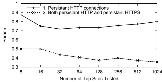
Figure 6: The applicability of the injection attacks on various sites.
