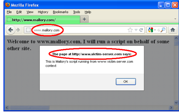
Figure 5: An XSS Attack. Mallory runs a script in context of www.victim-server.com within Mozilla Firefox sandbox. The address bar indicates the user is at www.mallory.com, but the message box context indication shows that the script (that Mallory provided) runs from www.victim-server.com.
