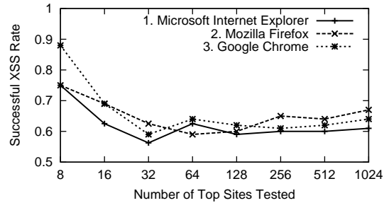
Figure 7: Rate of successful XSS attacks on connections to popular sites.
