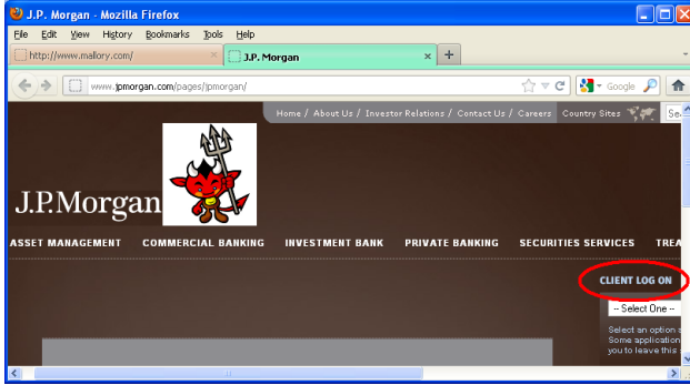
Figure 8: Web Spoofing/Defacement Attack. Mallory waits for the user to enter J.P. Morgan bank website, when he enters he injects a phony page. In this figure Mallory added a devil image.
