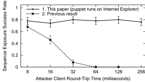
Figure 9: Comparison of sequence exposure techniques. Each measurement is the average of 50 runs, error bars mark standard deviations.
