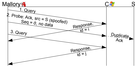
Figure 2: Server-Sequence Test.
