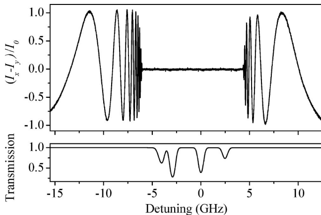
Fig. 2. Normalized Faraday signal as a function of detuning from ^{85}\text{Rb} F = 2 to F' = 3 obtained using a cell heated to 124 °C with an \sim 270 G applied magnetic field. A room temperature Doppler-broadened transmission spectrum is shown for reference.
