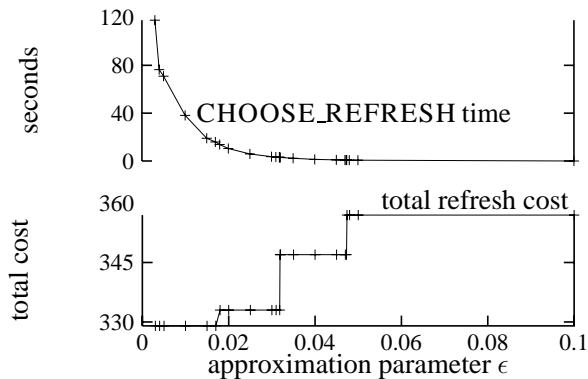
Figure 5: \text{CHOOSE\_REFRESH}_{\text{NO\_SEL/SUM}} time and refresh cost for varying \epsilon .
