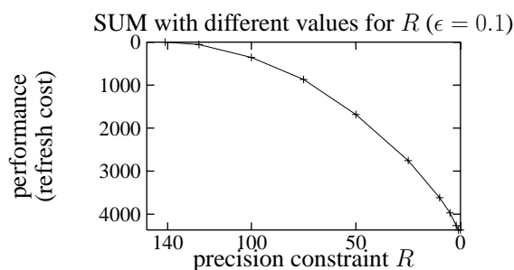
Figure 6: Precision-performance tradeoff for \text{CHOOSE\_REFRESH}_{\text{NO\_SEL/SUM}} .
