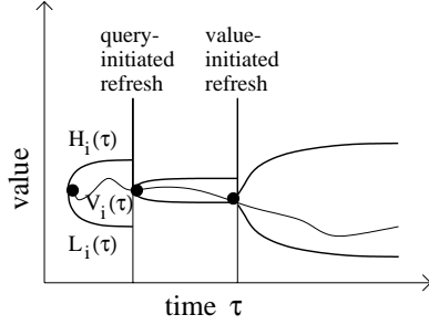
Figure 4: Bound [L_i(\mathcal{T}), H_i(\mathcal{T})] over time, overlaid with precise value V_i(\mathcal{T}) .
