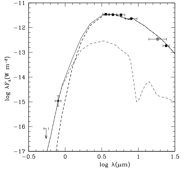
Fig. 6. Spectral energy distribution of BLG-360 in May 2006–August 2007. Symbols: V upper limit and I measurement (asterisk) from OGLE, Spitzer IRAC and MIPS measurements (full circles), as well as the AKARI measurement (open circle). See text for more details. Curves: model results obtained with the parameters listed in the third row of Table 1.
