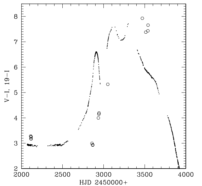
Fig. 2. Evolution of the V - I colour of OGLE-2002-BLG-360 – open symbols. The I curve of the object is also shown with small dots.
