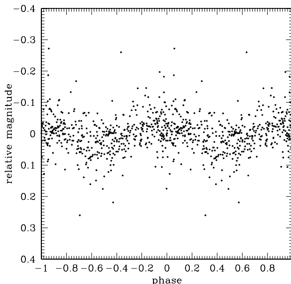
Fig. B.3. Photometric measurements of the progenitor of BLG-360 in 1995–99 folded with a period of 240 days, which corresponds to the highest peak in the power spectrum presented in Fig. B.2.
