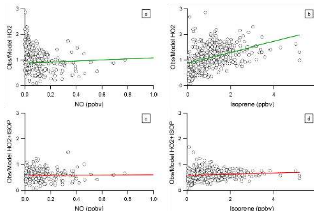
Fig. 9. Daytime (6 a.m.–9 p.m.) measured HO 2 * / modeled HO 2 (top) and measured HO 2 * /modeled HO 2 + ISOP (bottom), plotted versus NO (left) and isoprene (right) during CABINEX 2009. Unweighted linear correlations are shown in red and green.
