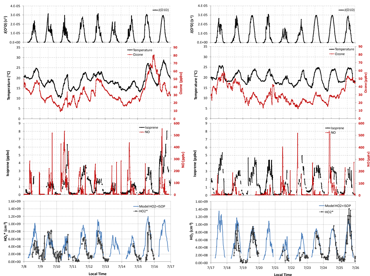
Fig. 1. PROPHET 2008 data showing key model constraints and modeled and measured \text{HO}_2^* concentrations. Measured \text{HO}_2^* precision (not shown) is approximately 1.5 \times 10^7 \text{ cm}^{-3} .
