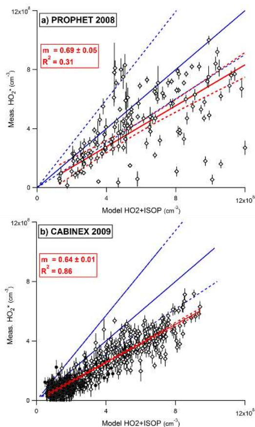
Fig. 4. HO 2 * correlation plots for PROPHET 2008 (top) and CABINEX 2009 (bottom, open diamonds = daytime, filled circles = nighttime) showing 30 s measurement values (sampled every 30 min) from each year. The blue lines are the 1 : 1 correlation (solid) and the model HO 2 + ISOP uncertainty (2σ) is shown by the dashed blue lines. The solid red line is a linear regression of the data with 95 % confidence limits shown as dashed red lines. Measurement precision for both years is approximately 1.5 \times 10^7 cm -3 .
