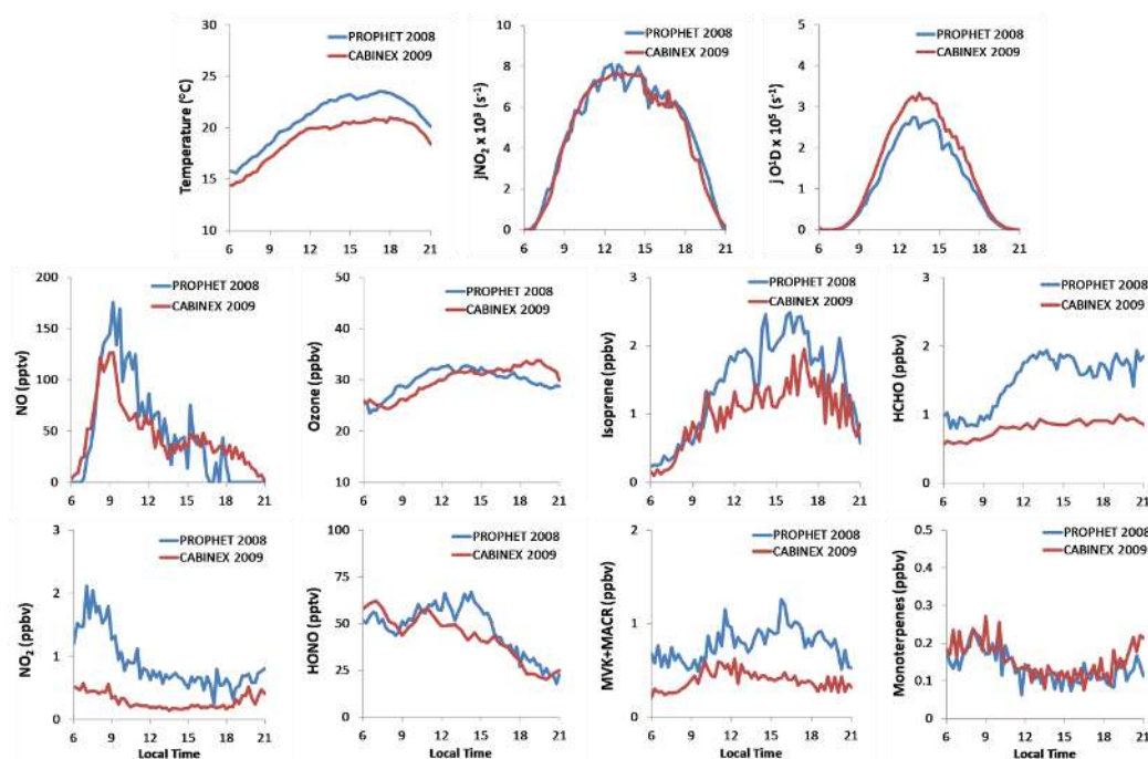
Fig. 3. Diel median values of several species measured from above canopy during PROPHET 2008 (blue) and CABINEX 2009 (red). Constrained model inputs based on overlap of measurements are shown in the Supplement.
