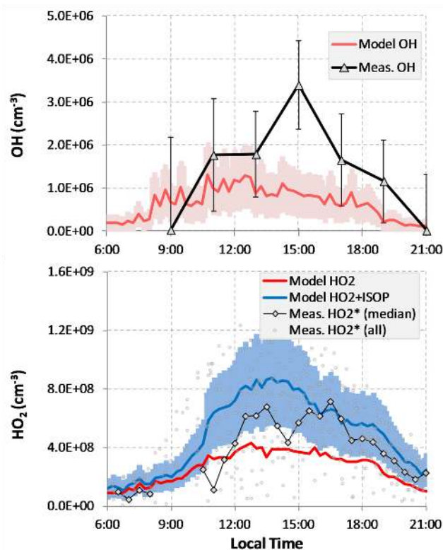
Fig. 5. PROPHET 2008 OH and HO 2 * median measurements with the RACM/MIM model results. Measured points are shown as 2 h medians (OH, triangles) and 30 min medians (HO 2 *, diamonds) for the daytime measurements (6 a.m.–9 p.m.). Error bars are the 2σ measurement precision for OH, while the HO 2 * measurement precision (not shown) is approximately \pm 2.0 \times 10^7 cm -3 . Gray circles in the bottom plot represent all of the HO 2 * measurements during PROPHET 2008 while the gray diamonds are the 30 min median for the times of this analysis where HO 2 * measurements are available. The red lines represent the base RACM/MIM daytime model results for OH (2σ relative uncertainty \pm 50 % shaded) or HO 2 . The blue lines represent the daytime modeled HO 2 + ISOP (2σ relative uncertainty \pm 33 % shaded).
