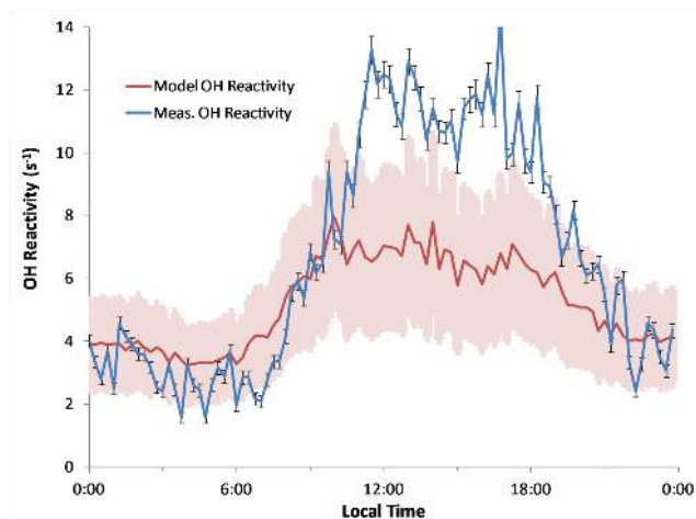
Fig. 8. Measured and modeled median total OH reactivity for the period analyzed for CABINEX 2009 (26 July–8 August). Error bars on the measured points are the 2\sigma uncertainty values ( \pm 3\% + 0.14 \text{ s}^{-1} , 50 point median). Pink outline is the 2\sigma uncertainty ( \pm 40\% ) of the modeled OH reactivity.
