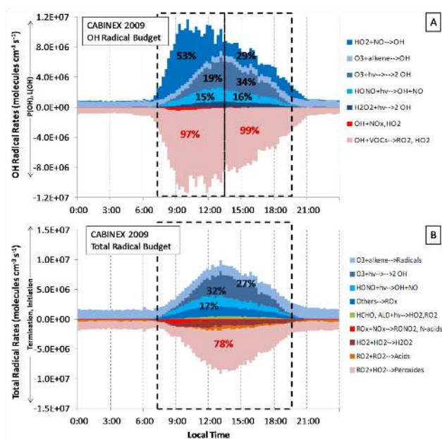
Fig. 12. CABINEX 2009 radical budget diagrams showing the campaign median OH radical budget (A) that compares all the production and loss terms (i.e., initiation, termination, and propagation routes) for OH and the total radical budget (B) that groups and compares all initiation and termination reaction rates for OH, HO 2 , and RO 2 radicals.
