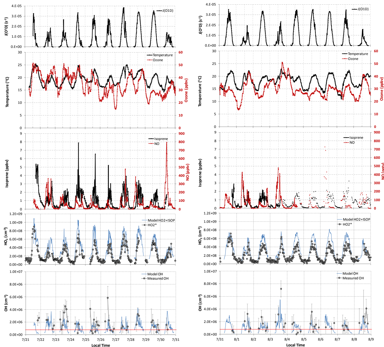
Fig. 2. CABINEX 2009 data showing key constraints and modeled and measured OH and HO 2 * concentrations. Error bars on the OH measurements are the 1 \sigma precision values of each measurement. Measured HO 2 * precision (not shown) is approximately 1.5 \times 10^7 cm -3 . The red line in the OH plot indicates the LOD on the 2 h median measurements ( 1.0 \times 10^6 cm -3 ). Only positive daytime OH measurements are shown for simplicity.
