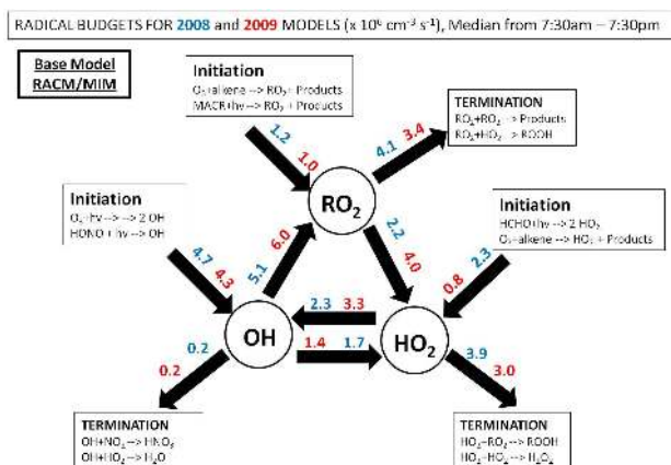
Fig. 10. PROPHET 2008 (blue) and CABINEX 2009 (red) radical budget rates for the time period of 7.30 a.m.–7.30 p.m. Primary reactions contributing to the initiation, termination, and propagation routes are shown in the boxes.
