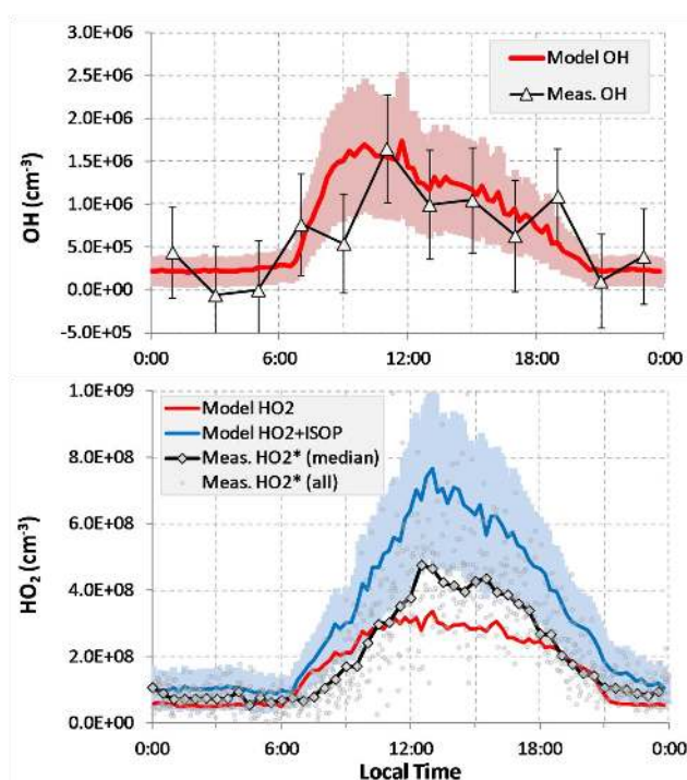
Fig. 7. CABINEX 2009 OH and \text{HO}_2^* median measurements with the RACM/MIM model results. Measured points are shown as 2 h medians (OH, triangles) and 30 min medians ( \text{HO}_2^* , diamonds). Error bars are the 2\sigma measurement precision for OH, while the \text{HO}_2^* measurement precision (not shown) is \pm 1.5 \times 10^7 \text{ cm}^{-3} . Gray points in the bottom plot represent the entire above canopy \text{HO}_2^* measurements during CABINEX 2009. The red lines represent the base RACM/MIM model results for OH ( 2\sigma relative uncertainty \pm 32\% shaded) or \text{HO}_2 . The blue lines represent the modeled \text{HO}_2 + \text{ISOP} ( 2\sigma relative uncertainty \pm 30\% and \pm 41\% shaded for day and night).
