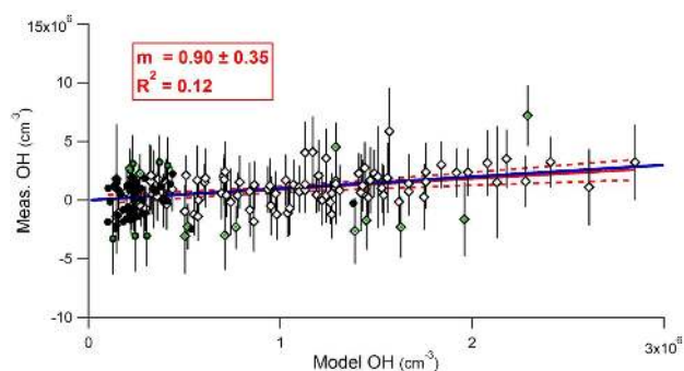
Fig. 6. OH correlation plot for CABINEX 2009 (filled circles = nighttime, open diamonds = daytime) showing 2 h median values. Vertical error bars are 2\sigma precision values on the measurements. The CABINEX 2\sigma model uncertainty (40 %) is excluded. Green points are significantly ( 2\sigma ) outside of the error bar range. Night-time points within the 2\sigma uncertainty do not have their precision values shown. The blue line is a 1 : 1 correlation line and the solid red line shows a measurement vs. model regression of the data weighted by the precision in the measurements and the uncertainty of the model concentrations (slope = 0.90 \pm 0.35 ), with dashed red lines representing the 95 % confidence limits of the slope.
