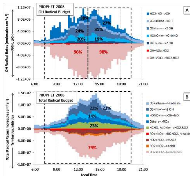
Fig. 11. PROPHET 2008 radical budget diagrams showing the campaign median OH radical budget (A) that compares all the production and loss terms (i.e., initiation, termination, and propagation routes) for OH and the total radical budget (B) that groups and compares all initiation and termination reaction rates for OH, \text{HO}_2 , and \text{RO}_2 radicals.
