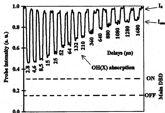
FIG. 4. Experimental resonant absorption result in saturated argon-water vapor mixture at atmospheric pressure.
