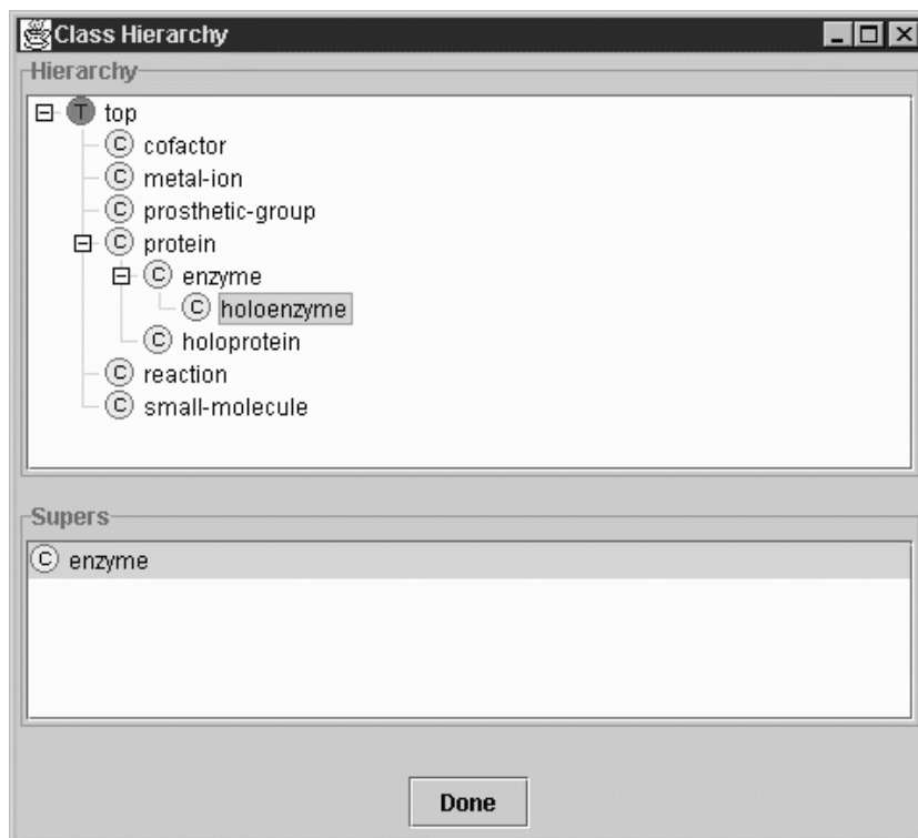
Fig. 3. Hierarchy pre-classification
