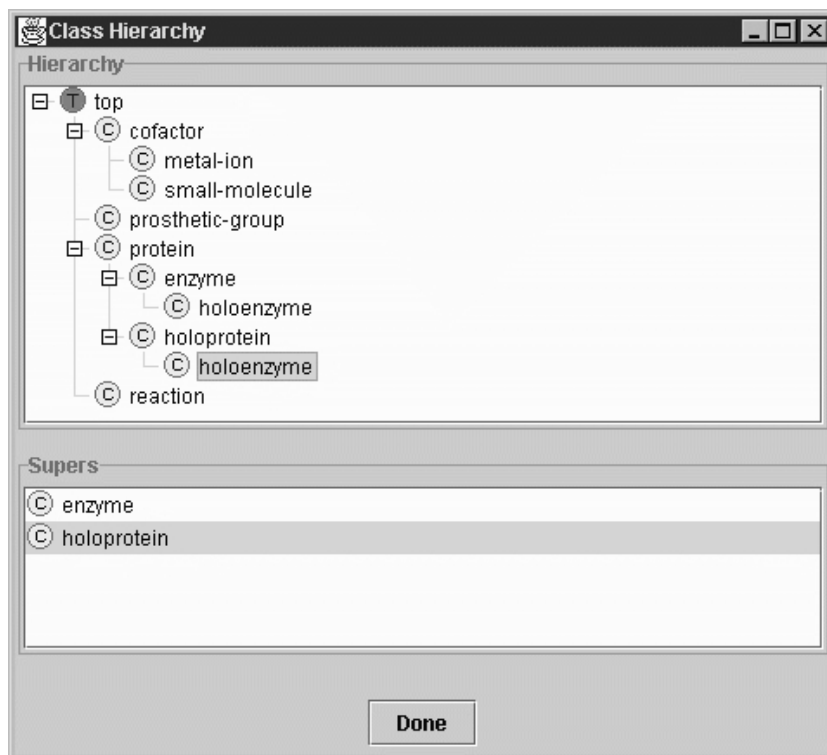
Fig. 4. Hierarchy post-classification
