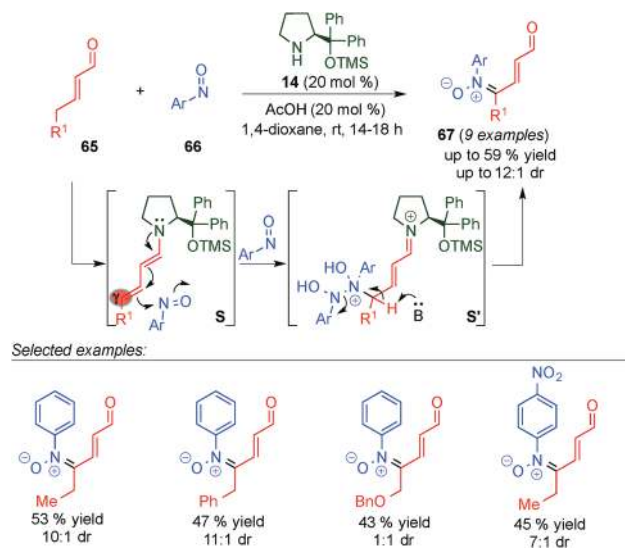
Scheme 17 \gamma -Site-selective addition of nitron to \alpha,\beta -unsaturated aldehydes.
