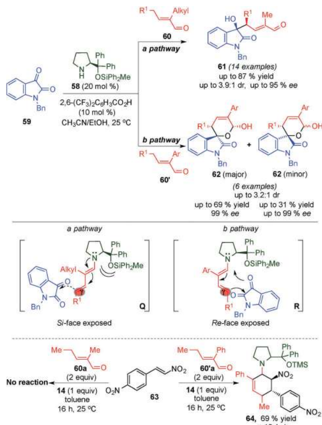
Scheme 16 \gamma -Site-selective aldol reaction between \alpha -branched enals and isatin via dienamine activation.
