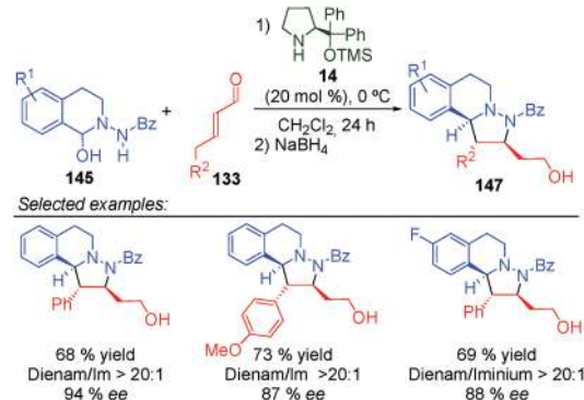
Scheme 42 First examples of [3+2] cycloaddition via dienamine activation.
