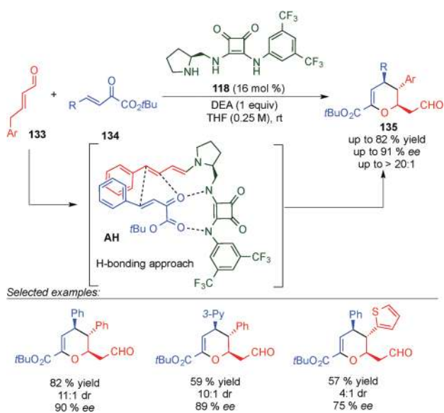
Scheme 37 First H-bond controlled dienamine-mediated catalytic inverse-electron demand Diels-Alder reaction.
