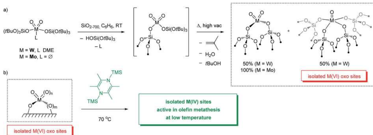
Scheme 8 Preparation (a) and activation (b) of molecularly-defined isolated M(\text{VI}) oxo ( M = \text{W} or \text{Mo} ) sites on silica.
