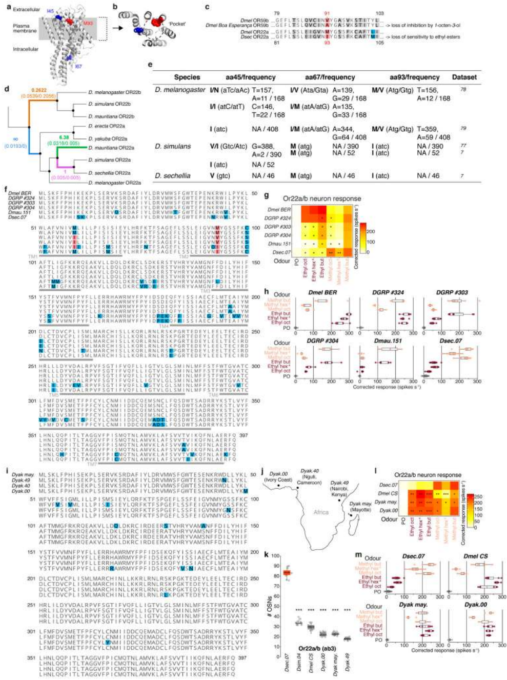
Extended Data Fig. 11. Phylogenetic and functional analysis of odour-specificity determinants in OR22a.
