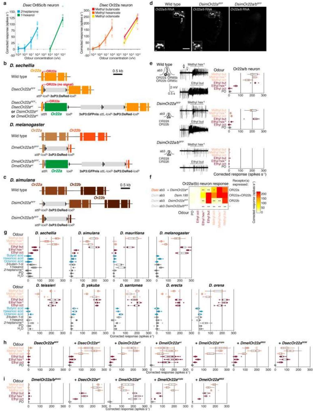
Extended Data Fig. 8. Odour-tuning properties of drosophilid Or85c/b and Or22a(b) neurons and genomic modifications of the Or22a(b) loci.
