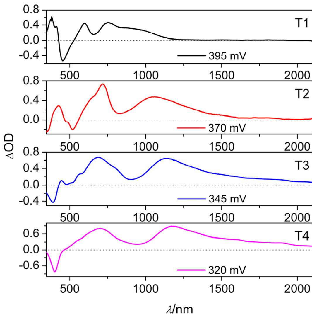
Fig. S3 Absorption change upon applying a positive potential bias (versus ferrocene) to a dye-coated titania film immersed in EMITFSI.
