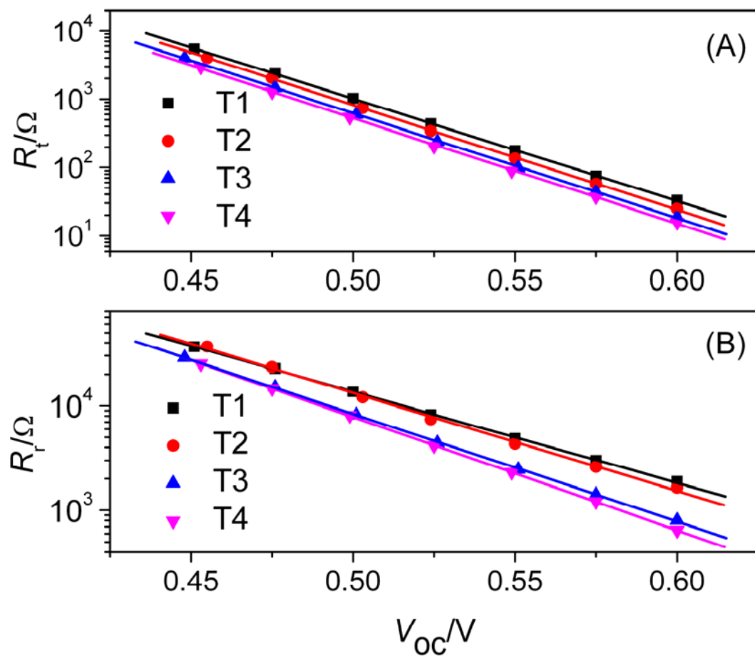
Fig. S5 Plots of (A) electron transport resistance and (B) interfacial charge recombination resistance versus the applied potential bias which is equal to the value of V_{oc} in impedance measurements. The solid lines are fittings in terms of proper functions.
