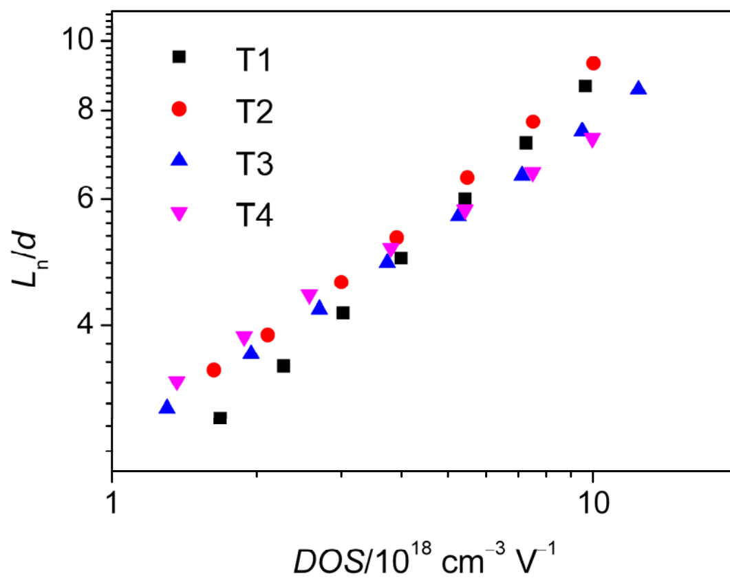
Fig. S2 The ratio of electron diffusion length ( L_n ) derived from impedance measurements relative to the titania film thickness ( d ).
