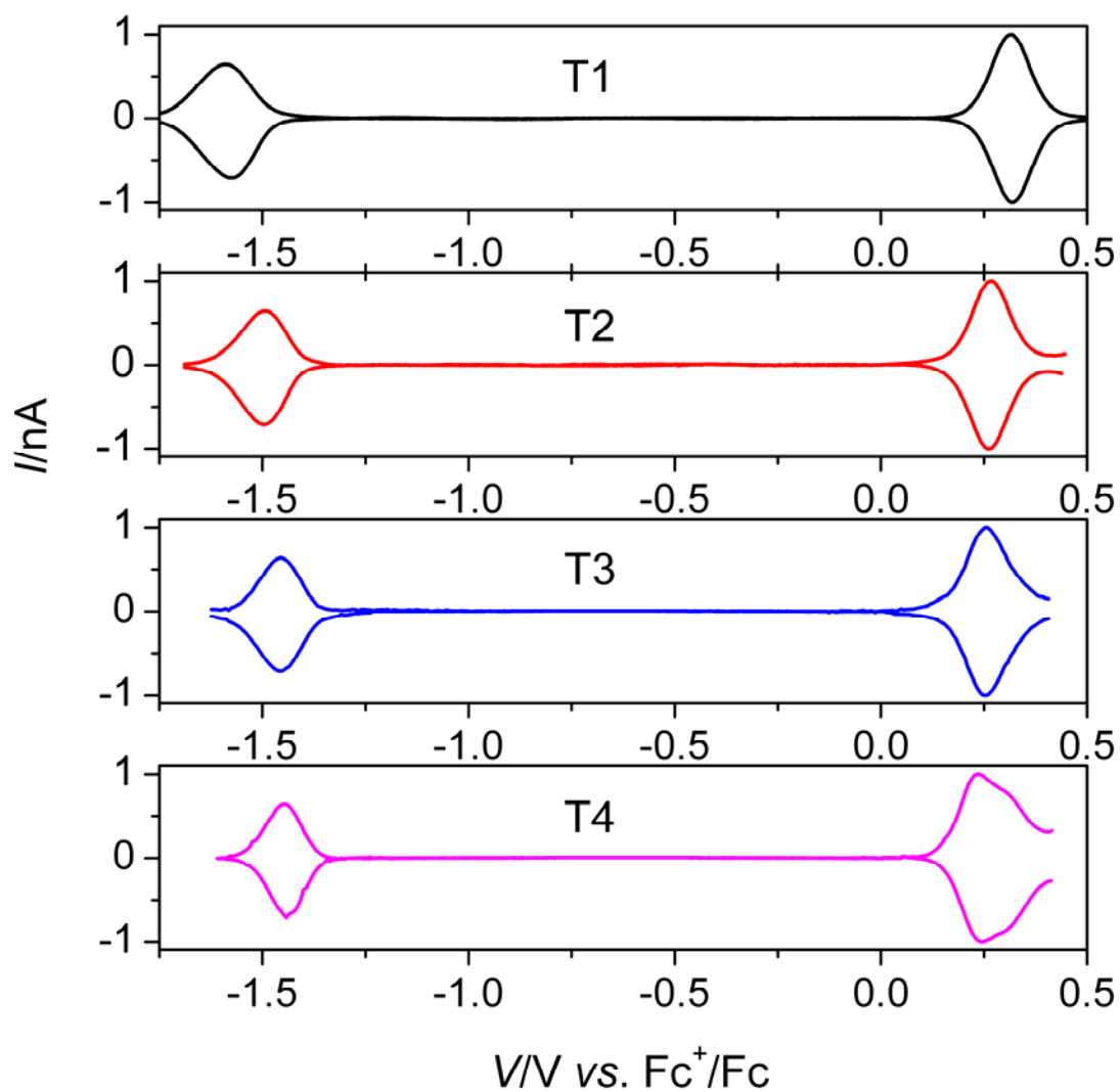
Fig. S4 Square-wave voltammograms of T1–T4 dissolved in N,N -dimethylformamide with 0.1 M tetra- n -butylammonium hexafluorophosphate as the supporting electrolyte.
