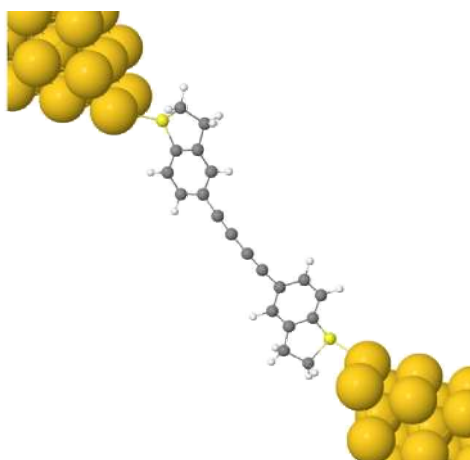
Figure S2. An example of molecule (ie oligoynes with length N = 2 with BT anchor) in a junction between two gold electrodes. The Sulfur atoms in BT anchors are connected to the gold electrodes.
