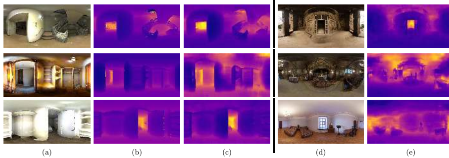
Fig. 1: We learn the task of predicting depth directly from omnidirectional indoor scene images. Results from our RectNet model are presented (left to right): (a) 360^\circ image samples from our test set, (b) corresponding ground truth depth, (c) predicted depth maps of the test image samples, (d) 360^\circ unseen image samples from the Sun360 dataset, (e) predicted depth maps of the Sun360 image samples.
