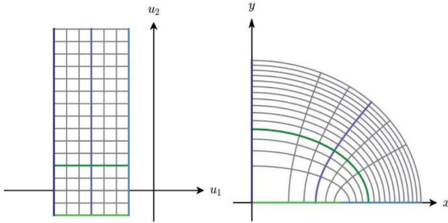
FIG. 3. Square grid on the domain \mathcal{U} and its image under the map (47). The horizontal lines u_2 = \text{const} are mapped to ellipses with the degenerate case u_2 \searrow -b , which is mapped to a line segment on the x -axis. The vertical lines u_1 = \text{const} are mapped to hyperbolas with the degenerate cases u_1 \nearrow -b , which is mapped to a ray on the x -axis, and u_2 \searrow -a , which is mapped to the positive y -axis.
