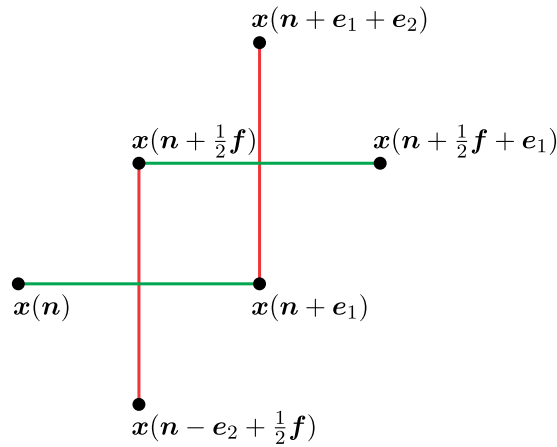
FIG. 6. Combinatorics of the factorization property (52).
