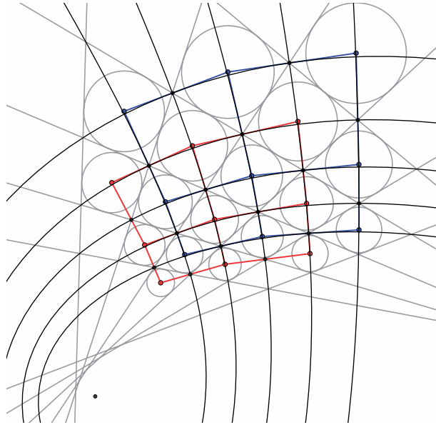
FIG. 8. Two dual subnets \eta and \tilde{\eta} of the net of incentres of an IC-net. The edges are tangent to confocal conics, and corresponding edges of the two nets are orthogonal.
