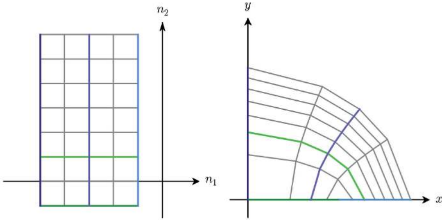
FIG. 4. Points of the square grid on the domain \mathcal{U} and their images under the map (48), joined by straight line segments respectively. The horizontal lines n_2 = \text{const} are mapped to discrete ellipses with the degenerate case n_2 = -\beta , which is mapped to a line segment on the x -axis. The vertical lines n_1 = \text{const} are mapped to discrete hyperbolas with the degenerate cases n_1 = -\beta , which is mapped to a ray on the x -axis, and n_1 = -\alpha , which is mapped to the positive y -axis.
