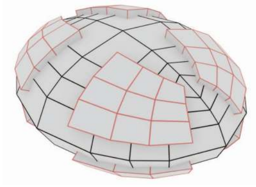
FIG. 7. A discrete ellipsoid ( n_1, n_2 integer, n_3 = \text{const} ) from the system (53) and its two adjacent layers from the dual n ( n_1, n_2 half-integer, n_3 = \text{const} \pm \frac{1}{2} ). All faces are planar and orthogonal to the corresponding edges of the other net.
