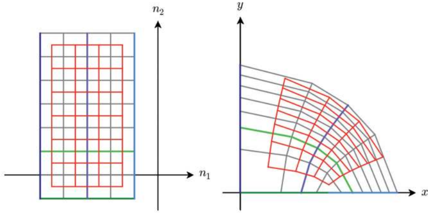
FIG. 5. Points of the square grid on the domain \mathcal{U} \cup \mathcal{U}^* and their images under the map (48). All pairs of corresponding dual edges are mutually orthogonal.
