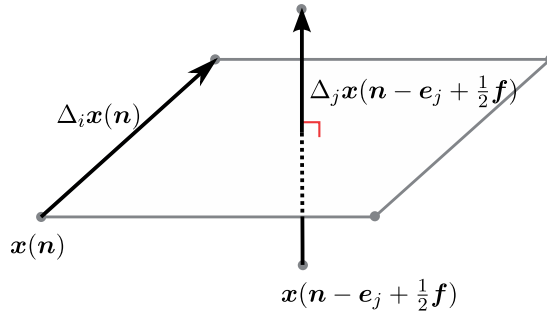
FIG. 2. Discrete orthogonality for a system of Q-nets defined on a square lattice and on its dual.
