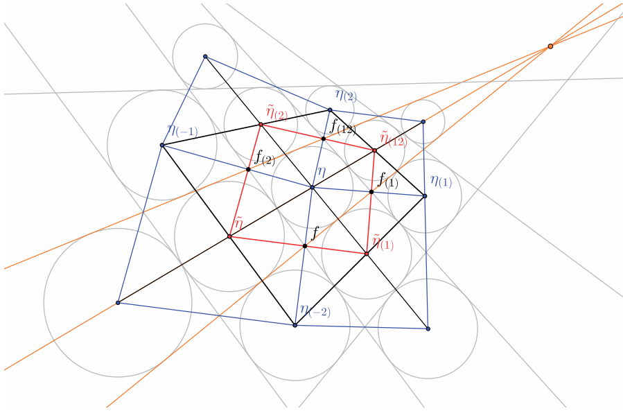
FIG. 9. Koenigs property of the incentre net \omega of an IC-net implies the Koenigs property for its two diagonal nets \eta and \tilde{\eta} .
