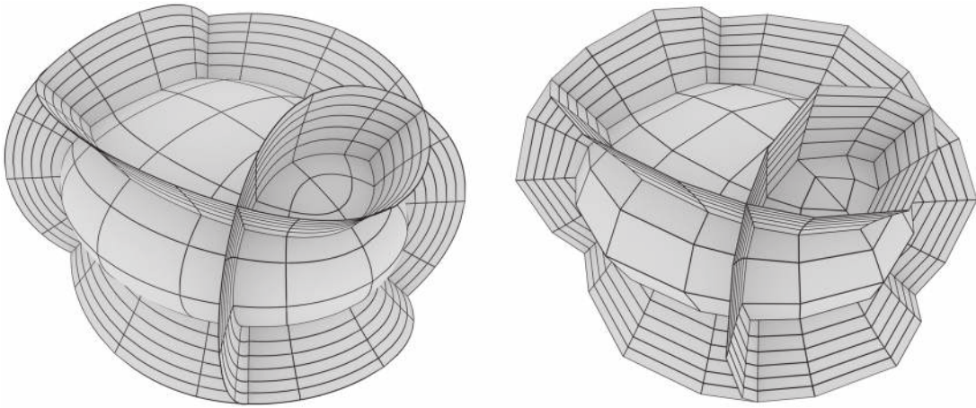
FIG. 1. Left: three quadrics of different signature from a family of confocal quadrics in \mathbb{R}^3 . Right: the corresponding three discrete quadrics from a family introduced in the present article.
