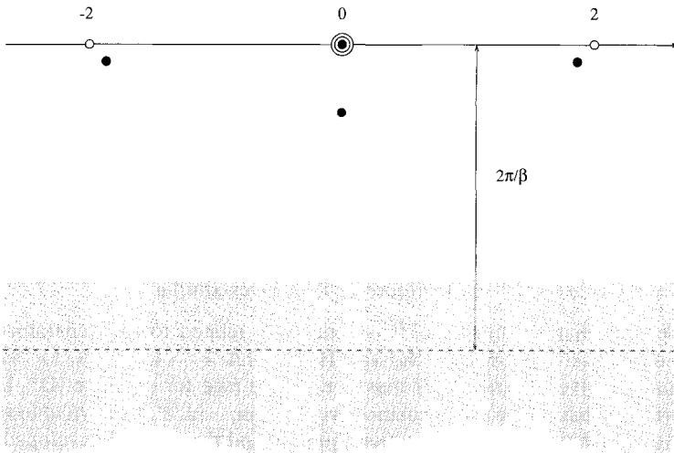
Fig. 1. The eigenvalues of L_0 (white discs) and the resonances of L_{\lambda} (black discs). The complex translation moves the essential spectrum of the Liouvillian into the shaded area. The first singularity of the function \alpha_{\beta} in the lower half-plane lies on the dotted line
