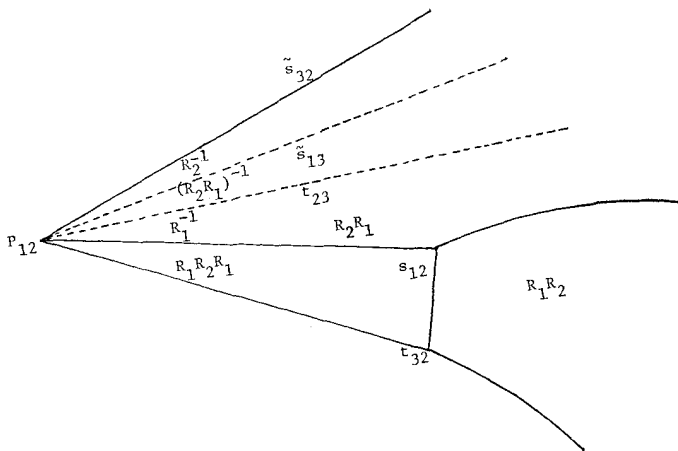
FIGURE 10.2. F_{12} \cap \widehat{R}_1
