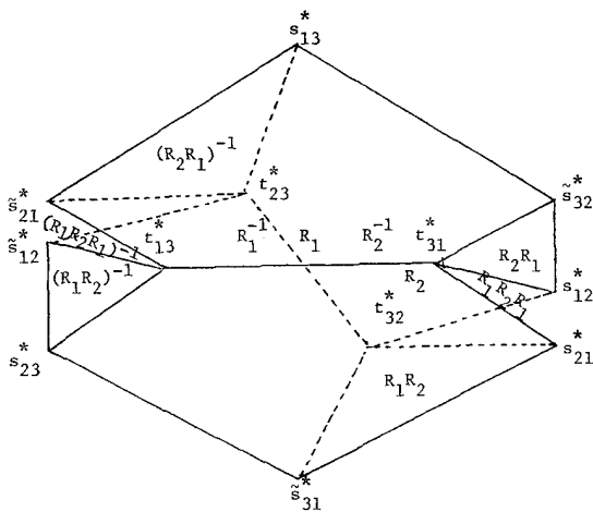
FIGURE 10.1. The intersection F_{12}^* of F_{12} with a 3-sphere S_r centered at p_{12} of radius r=d(p_{12}, p_0) .
