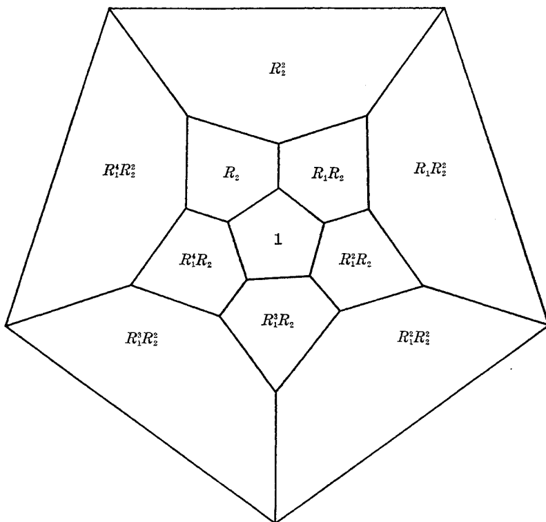
FIGURE 7.2c. p=5 : Representatives for \Gamma_{12}/\Gamma_1Z The bottom face represents the coset R_2^{-1}R_1^2R_2^2\Gamma_1Z .
