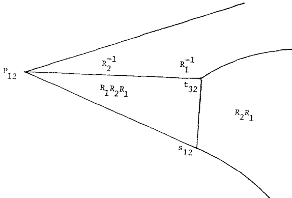
FIGURE 10.3. F_{12} \cap (\widehat{R}_1 \widehat{R}_2)
