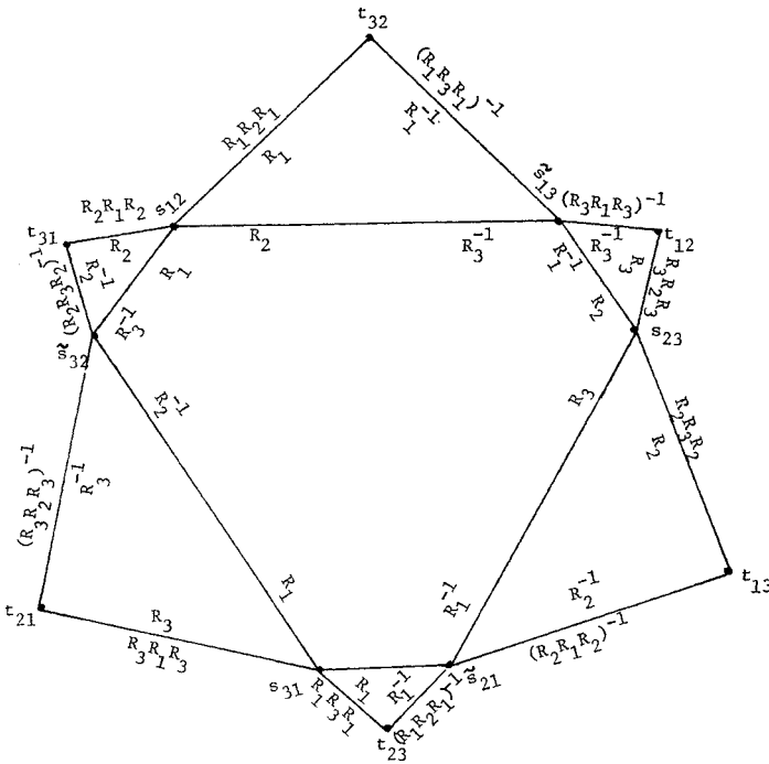
FIGURE 14.1. A schematic drawing of \Delta_{ijk} = I_{ijk} \cap F(\varphi) for |\arg \varphi^3| < \pi/2 - \pi/p . As \varphi^3 \rightarrow \bar{\eta}i , \Delta_{321} approaches the point at \infty . For \arg \varphi^3 > \pi/2 - \pi/p , \Delta_{321} becomes a single (finite) point in the ball so long as \arg \varphi^3 < 3(\pi/2 - \pi/p) . For -3(\pi/2 - \pi/p) < \arg \varphi^3 \leq -(\pi/2 - \pi/p) , \Delta_{123} is a single point.
