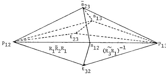
FIGURE 14.2. The nine faces of \tilde{R}_1 (labeled by the intersecting 3-faces) for |\arg \varphi^3| < \pi/2 - \pi/p .
