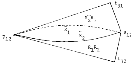
FIGURE 14.4. The four faces of R_1\tilde{R}_2R_3 for |\arg \varphi^3| < \pi/2 - \pi/p .
