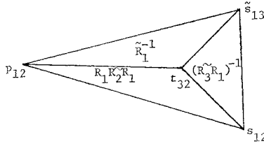
FIGURE 14.3. The four faces of \tilde{R}_1\tilde{R}_2 for -(\pi/2 - \pi/p) < \arg \varphi^3 < 3(\pi/2 - \pi/p) .
