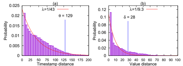
Figure 9: Distribution of (a) timestamp distances on consecutive tuples in dataset Fuel, which automatically determine time constraint \theta = 129 , and (b) value distances between aligned candidates and their model predictions, which automatically determine model constraint \delta = 28
