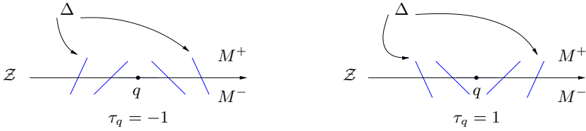
Figure 5.3. Tangency points with opposite contributions
