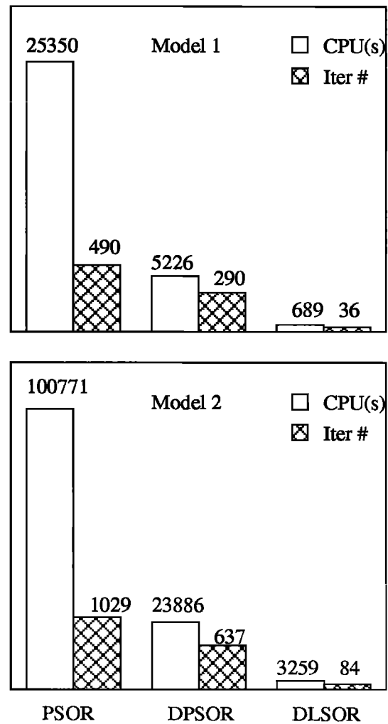
Figure 6. CPU time (in seconds) and average iteration number for each iterative relaxation procedure. The initial guess for the solution before each iterative procedure was a zero velocity field.
