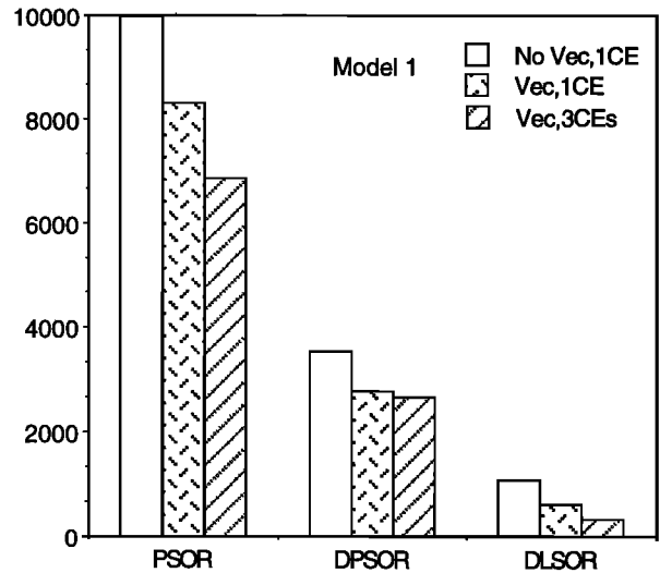
Figure 8. CPU time (in seconds) on one CE without vectorization, on one CE with full optimization, and on three CEs with full optimization. The initial guess for solution before each iterative procedure is the velocity field obtained at the previous time step.
