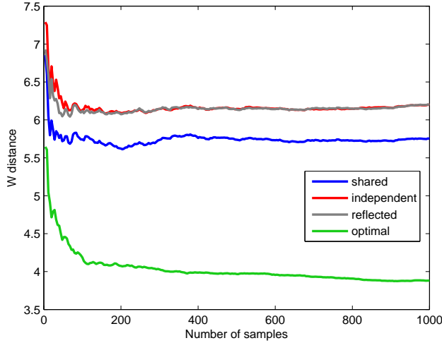
Figure 1: Evaluation of expected distances between x and \bar{x} depending on the number of samples, over different couplings: shared (blue line in the middle), independent and reflected noises (resp. red and gray lines on the top), optimal coupling (green line at the bottom).
