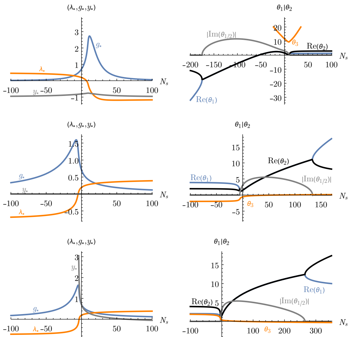
Figure 5. Illustration of the fixed point structure resulting from the full system of beta functions (3.13) as a function of N_s . The characteristics of the NGFP - , NGFP 0 , and NGFP + are shown in the first, second, and third row, respectively.
