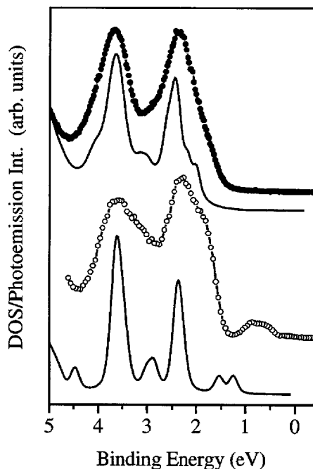
FIG. 3. Valence band photoemission spectra of (C_5 N)_2 ( \bullet ) and (Rb_1 C_{60})_2 ( \circ ) (spectra of the latter from Ref. [14]). The spectrum of dimerized Rb_1 C_{60} is shifted by 0.25 eV to lower binding energy. The solid lines are the calculated DOS for a C_5 N dimer and for a C_{60}^- dimer, respectively. For details, see text.
