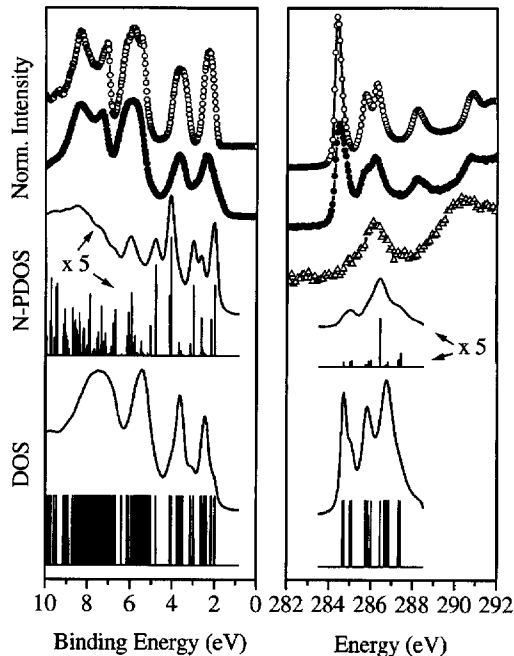
FIG. 1. Valence band photoemission spectra and C 1s core level excitation spectra of (C_5 N)_2 ( \bullet ), and C_{60} ( \circ ). Also shown is the N 1s excitation spectrum ( \Delta ) of the heterofullerene. At the bottom in each panel are both the calculated densities of states (DOS) and the broadened DOS for the C_5 N dimer and the DOS projected onto the N atomic functions (N-PDOS).
