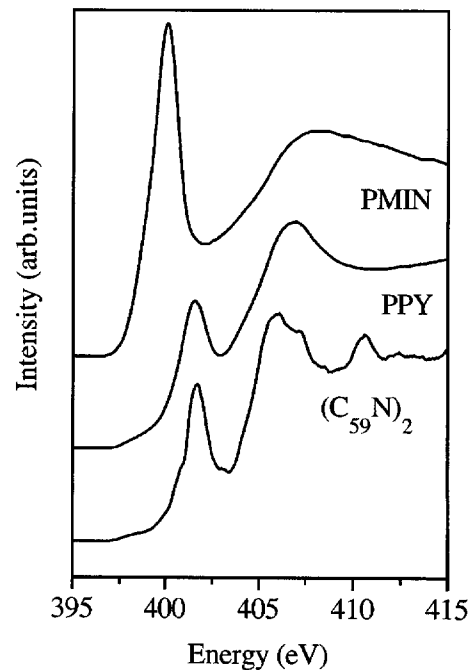
FIG. 4. Comparison of the N 1s excitation spectra of dimerized C_5 N , polypyrrole (PPY) [10] and polymethineimine (PMI) [10].
