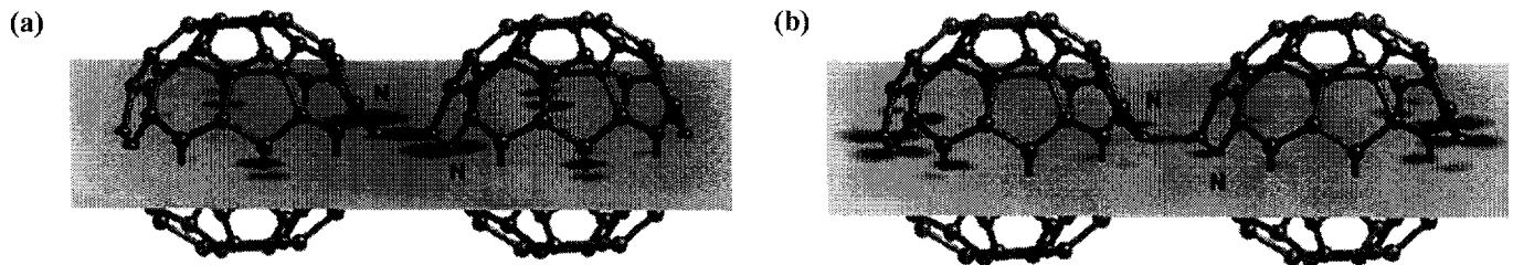
FIG. 2. A cut through the electronic density distribution of (a) the HOMO (left panel) and (b) the LUMO (right panel) of (C_5 N)_2 depicted in the plane passing through the N atoms and the intermolecular bond.
