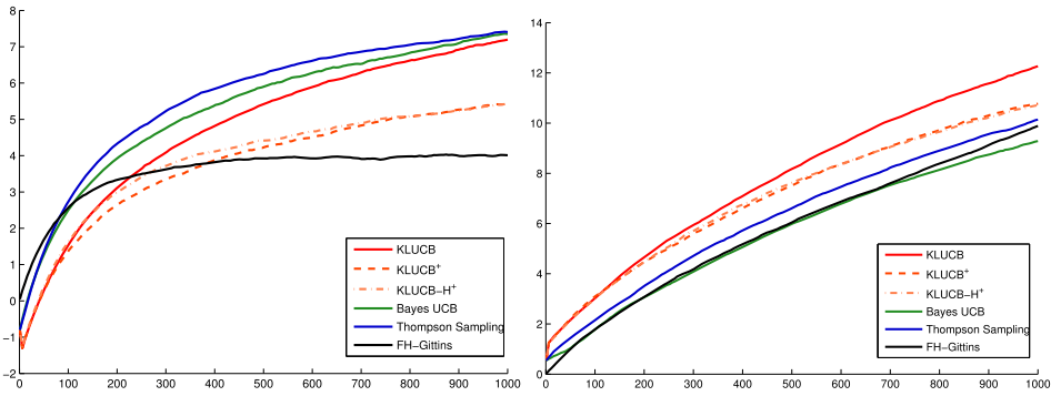
FIG. 2. Regret on two-armed Bernoulli bandits [ \mu = [0.05 \ 0.15] (left) \mu = [0.75 \ 0.8] (right)] up to horizon T = 1000 , averaged over N = 10,000 simulations.
