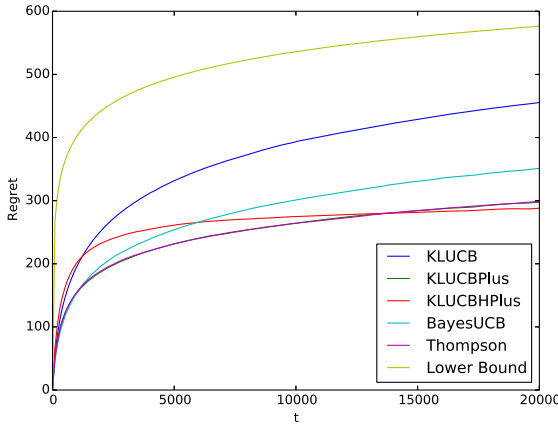
FIG. 3. Regret on a five-armed bandit with Exponential distributions with means \mu = [1 \ 1.5 \ 2 \ 2.5 \ 3] up to horizon T = 20,000 , averaged over N = 50,000 simulations.
