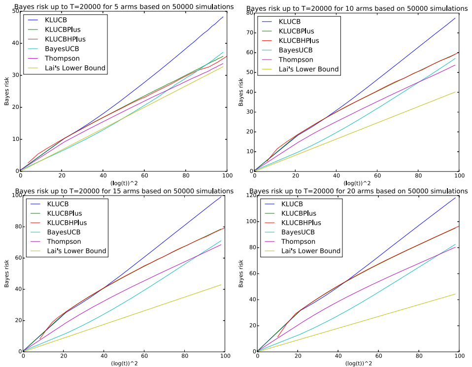
FIG. 4. Bayes risk up to T = 20,000 on a Bernoulli bandit model with a uniform prior on the K arms, for K = 5, 10, 15, 20 , averaged over N = 50,000 simulations.
