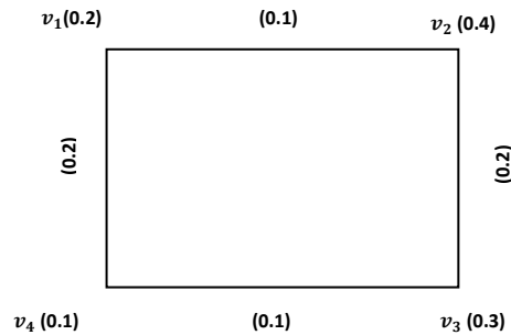
Figure 2: Fuzzy graph
